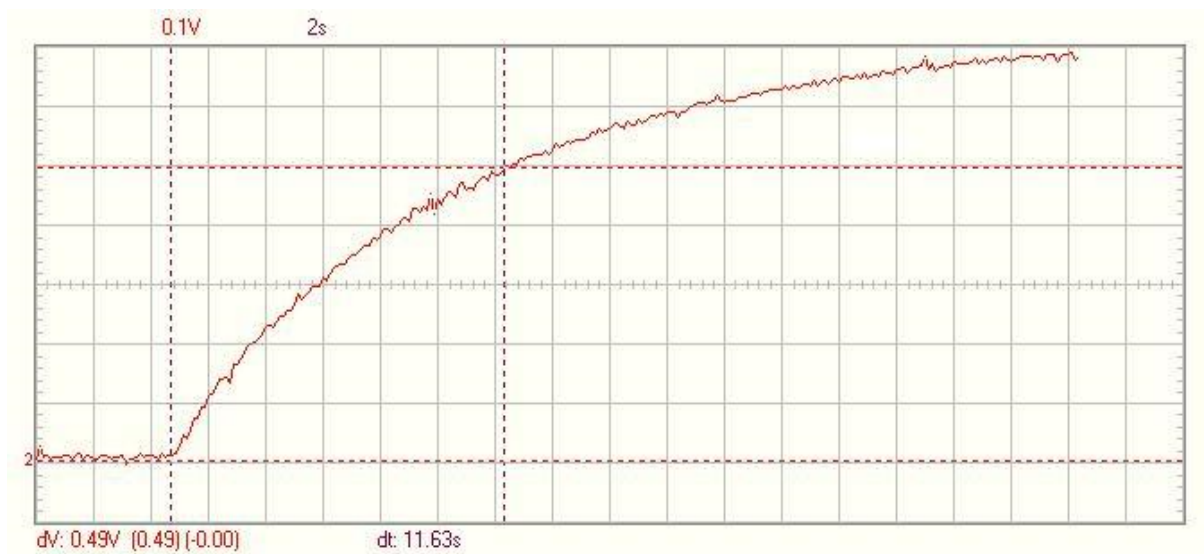
Fig. 5. Time characteristic graph of thermoelectric HFS with dimensions of 16 \times 16 \times 3 mm, equipped with ceramic receiving surface.
