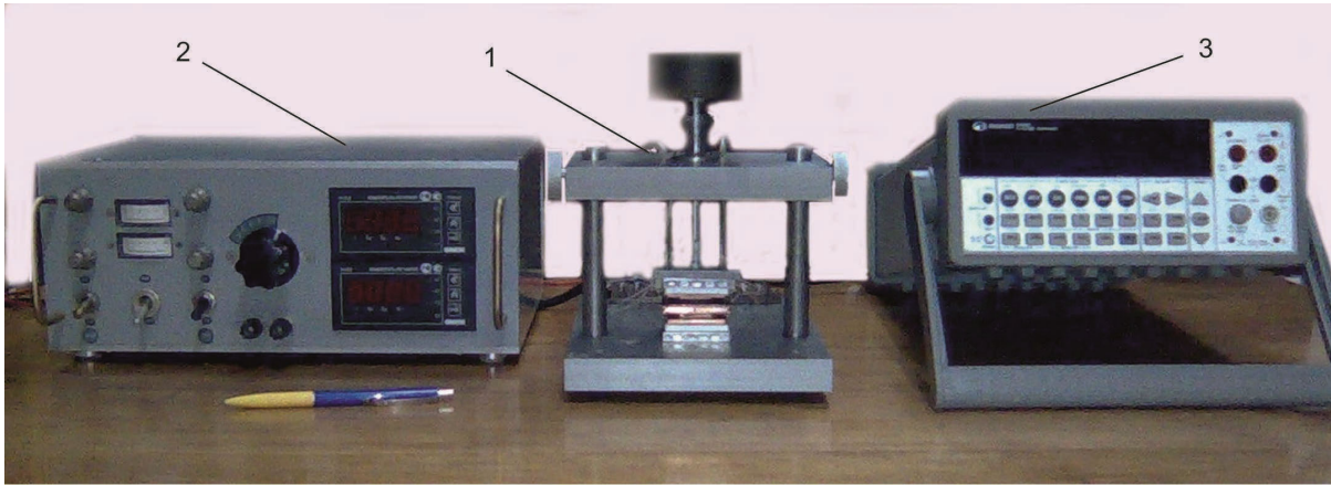
Fig. 1. Visual inspection of the bench for analysis of metrological properties and calibration of thermoelectric heat flux sensors (HFS).
