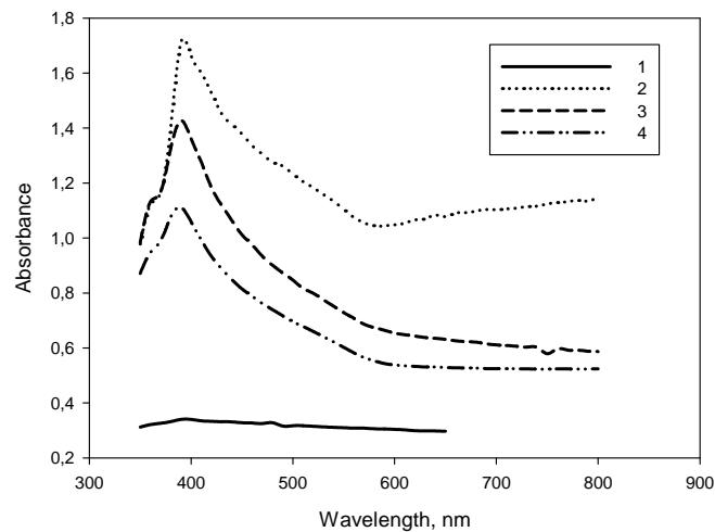
Fig. 3. Optical spectra of the chitosan-Cu films. 1 – Ch film; 2 – ChCu 20 s film; 3 – ChCu 15 s film; 4 - ChCu 10 s film; where 20, 15 and 10 s is the Cu deposition time
