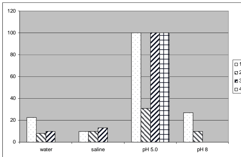
Fig. 4. Degradation of films (%) in different media (incubation for a month): 1 – Ch film; 2 – ChCu 20 s film; 3 – ChCu 15 s film; 4 – ChCu 10 s film
