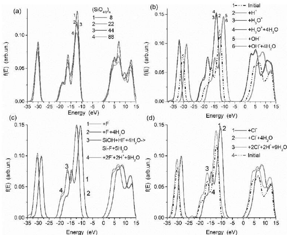
Fig. 8. Distribution functions of integral electron states of (a) neutral silica clusters with 8, 22, 44 and 88 units, (b) neutral and charged silica clusters (protonation of SiOH, addition of \text{H}_3\text{O}^+ alone or with 4 \text{H}_2\text{O} , binding of \text{OH}^- alone or with 4 \text{H}_2\text{O} ), (c) \text{F}^- and HF, (d) \text{Cl}^- and HCl alone or with addition of 4 or 9 water molecules ( b-d ) clusters with 44 units (method \omega\text{B97X-D/cc-pVDZ} )
