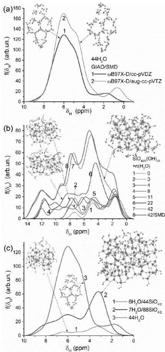
Fig. 6. ^1H NMR spectra calculated using the GIAO/ \omega B97X-D/cc-pVDZ (with or without SMD): (a) for water cluster with 44H 2 O with initial structure corresponding to ice Ih comparing to calculation using GIAO/SMD/ \omega B97X-D/aug-cc-pVTZ; (b) cluster with 43 units (formed from the cluster with 44 units by replacing Si with 4H) with different numbers of bound water molecules (0, 3, 4, 8, 11, 22, and 42); and (c) weakly hydrated clusters with 44 (+6H 2 O) and 88 (+7H 2 O) units and pure water cluster with 44H 2 O
