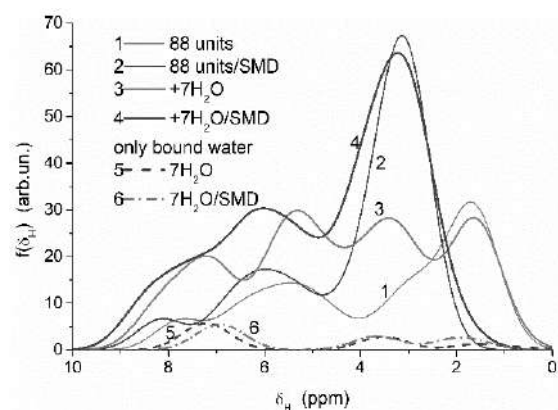
Fig. 7. ^1H NMR spectra calculated using the GIAO/ \omega B97X-D/cc-pVDZ (with (curves 2, 4, 6) or without (curves 1, 3, 5) SMD) for a silica cluster alone (curves 1 and 2) (88 units with 40OH) and with bound 7H 2 O (curves 3 and 4), and only for bound water (curves 5 and 6)
