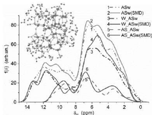
Fig. 9. ^1\text{H} NMR spectra of alumina/silica (11/33, 35OH) cluster with bound 42 \text{H}_2\text{O} (curves 1 and 2), only bound water (curves 3 and 4), and surface OH groups (curves 5 and 6) (DFT method with GIAO/ \omega B97X–D/cc–pVDZ, with (curves 2, 4, and 6) or without (1, 3, and 5) solvation effects with SMD)
