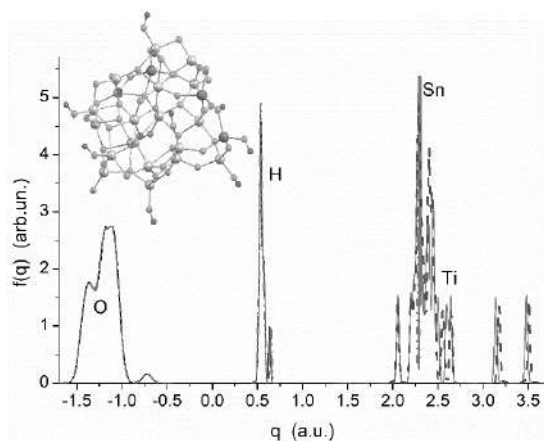
Fig. 5. Effects of the Sn/Ti ratio in the \text{SnO}_2/\text{TiO}_2 clusters ( \text{Sn}/\text{Ti} = 2/20 (dot-dashed lines) and 3/19 (solid lines) with 22 polyhedra (with 100H) on the atomic charge distribution functions for H, O, Ti, and Sn atoms (RHF with the DGDZVP basis set)
