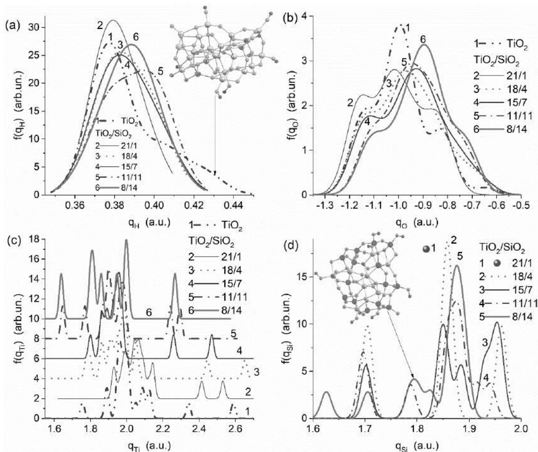
Fig. 1. Effects of the Ti/Si ratio in the TiO 2 /SiO 2 clusters with 22 polyhedra (with 10OH) of the initial anatase structure doped silicon dioxide on the atomic charge distribution functions for: (a) H, (b) O, (c) Ti, and (d) Si atoms (restricted HF (RHF) calculations with the 6-31G(d,p) basis set)
