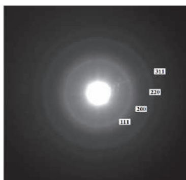
Fig. 3. Electronogram of particles in the nanocomposite is d(hkl) = 3.12 (111), 2.7 (200), 1.89 (220) and 1.64 Å (311)
