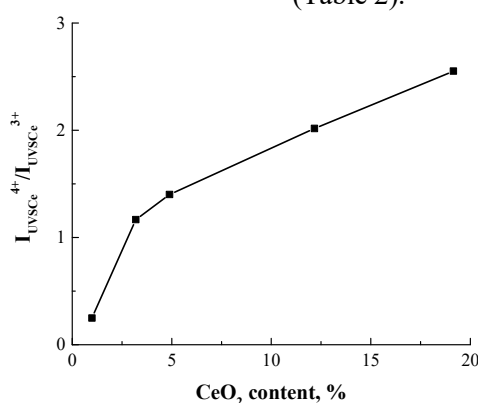
Fig. 9. Dependence of the ratio of the ratio of I_{UVScCe}^{4+}/I_{UVScCe}^{3+} on the content of \text{CeO}_2
