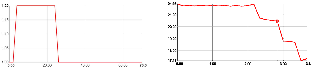
Fig. 3. Boundary conditions for the compression ratio (the dependence of compression ratio on time (hour)) at CS Borova (left). The boundary condition for CS Pervomaysk capacity (dependence of capacity (MW) on time (hour)) (right).
