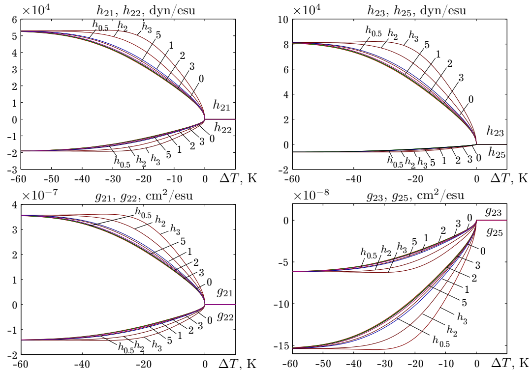
Fig. 13. Dependence of the piezoelectric voltage h_{2i} and strain g_{2i} constants on the temperature difference \Delta T = T - T_c : at ambient pressure — 0, at pressures of different symmetries, each with the magnitude of 0.5 GPa: uniaxial p_1 — 1, p_2 — 2, p_3 — 3, shear stress \sigma_5 — 5, and under hydrostatic pressure (GPa): 0.5 — h_{0.5} , 2 — h_2 , 3 — h_3 .
