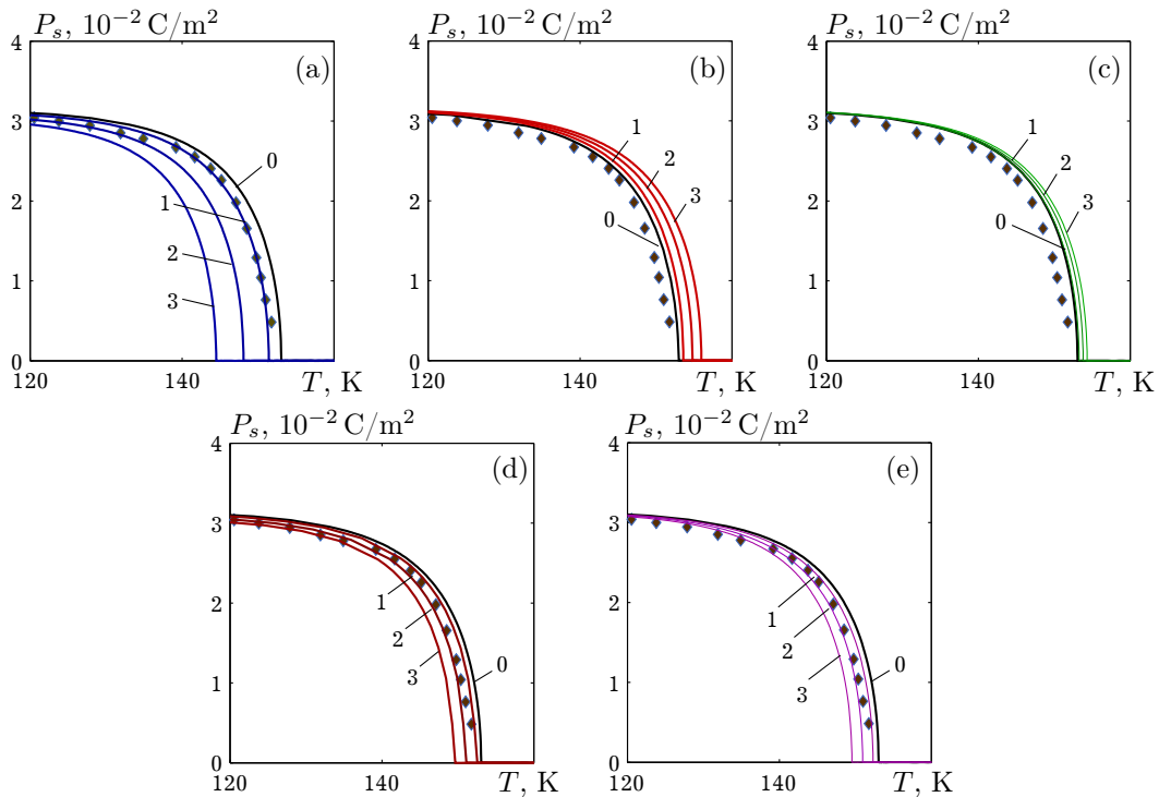
Fig. 4. The temperature dependence of spontaneous polarization of CDP under uniaxial pressures p_1 (a), p_2 (b), p_3 (c), hydrostatic pressure (d), shear stress \sigma_5 (e) of the following magnitudes (GPa): 0.0 – 0, \blacklozenge [1], 0.1 – 1, 0.3 – 2, 0.5 – 3.
