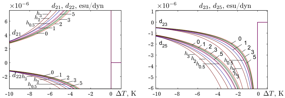
Fig. 12. Dependence of the piezoelectric strain coefficients d_{2i} on the temperature difference \Delta T = T - T_c : at ambient pressure — 0, at pressures of different symmetries, each with the magnitude of 0.5 GPa: uniaxial p_1 — 1, p_2 — 2, p_3 — 3, shear stress \sigma_5 — 5, and under hydrostatic pressure (GPa): 0.5 — h_{0.5} , 2 — h_2 , 3 — h_3 .
