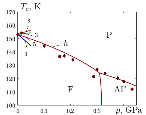
Fig. 2. Dependence of the temperature T_c of the transition between the paraelectric and ferroelectric phase of CDP on the uniaxial pressures p_1 - 1 , p_2 - 2 , p_3 - 3 , hydrostatic pressure p - h , \blacklozenge - [1] , \bullet - [5] and shear stress \sigma_5 - 5 .
