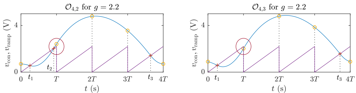
Fig. 18. Period-4 trajectories before border collision for g = 2.2 .
