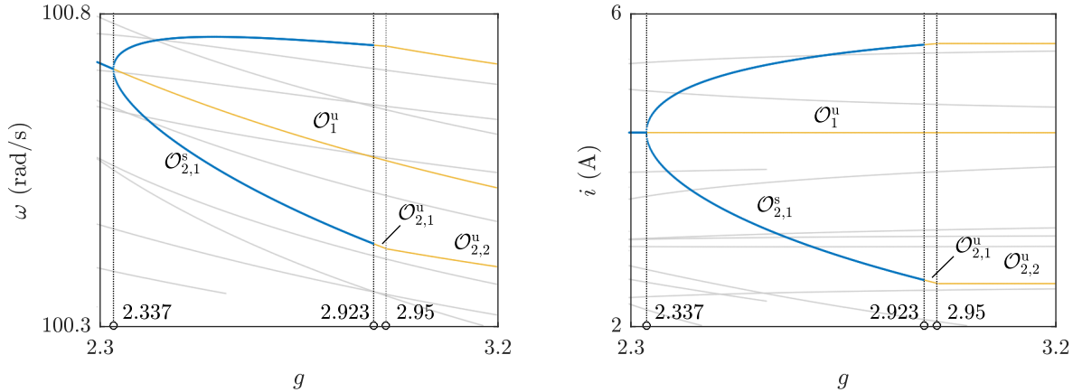
Fig. 7. Blow-up of Fig. 5 demonstrating period-2 orbits \mathcal{O}_{2,i} .
