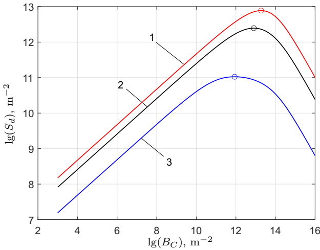
Fig. 2. Dependence of the sensitivity S_d of hydrodynamic bridge transducer on the design complex parameter B_C : 1, B_{P1} = 1.897082 \cdot 10^{-9} N; B_{P2} = 2.580313 \cdot 10^{-9} N; 2, B_{P1} = 1.021878 \cdot 10^{-9} N; B_{P2} = 1.997774 \cdot 10^{-8} N; 3, B_{P1} = 1.021878 \cdot 10^{-9} N; B_{P2} = 7.671857 \cdot 10^{-7} N.
