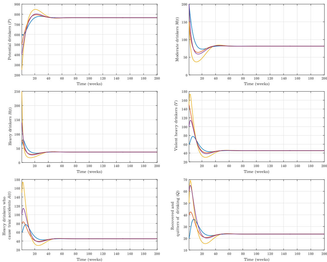
Fig. 5. Stability of alcohol present equilibrium E^* for different initial values of each variable state, when R_0 = 1.30 > 1 and with fixed value of fractional derivative \alpha = 0.1 .
