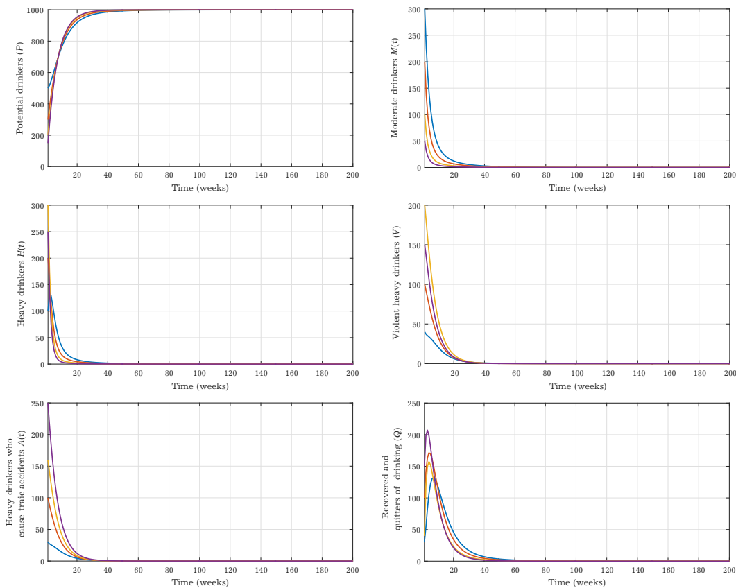
Fig. 4. Stability of drinking-free equilibrium E^0 for different initial values of each variable state, when R_0 = 0.87 < 1 and with fixed value of fractional derivative \alpha = 0.1 .
