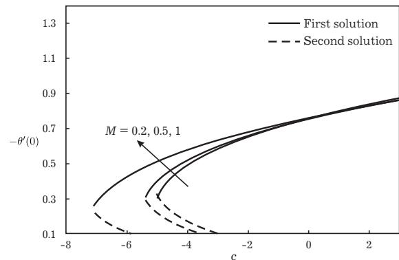
Fig. 4. Variation of -\theta'(0) with c for different values of M when A = 1 , K = 1 and Pr = 0.5 .
