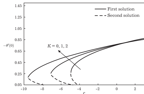
Fig. 6. Variation of -\theta'(0) with c for different values of K when A = 1 , M = 1 and Pr = 0.5 .
