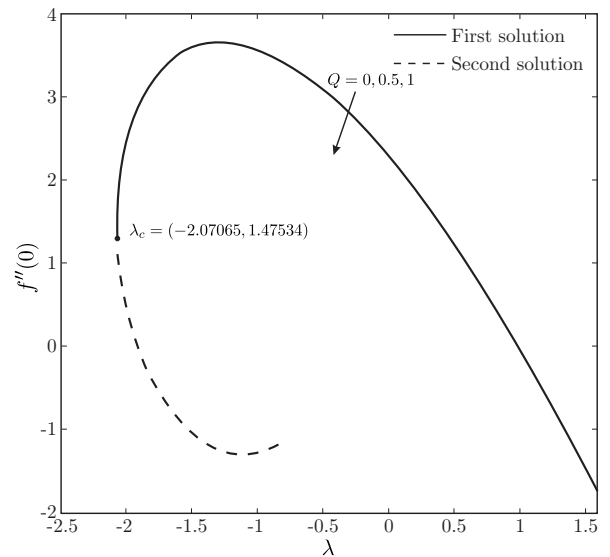
Fig. 3. Skin friction coefficient f''(0) of Q = 0, 0.5, 1 at Pr = 1, K = 0 and S = 1 .
