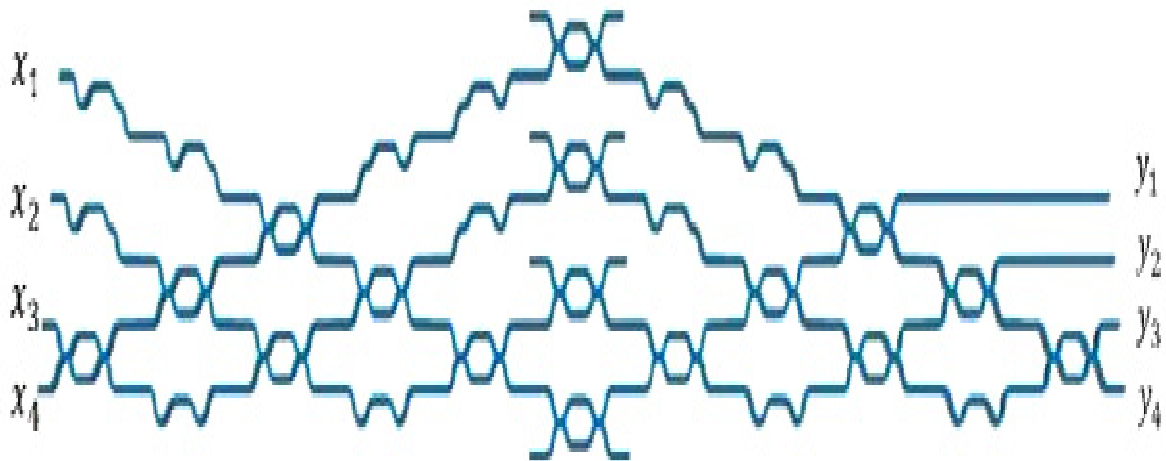
Figure 3 – MZI-MVM method
