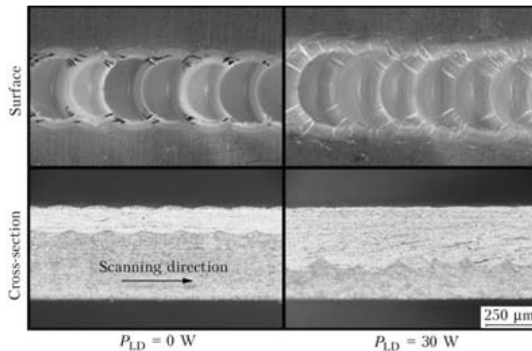
Figure 4. Surface and cross section of weld bead in bead-on-plate irradiation at scanning velocity v = 30 \text{ mm/s} , pulse duration of Nd:YAG laser \tau = 1.2 \text{ ms} , pulse repetition rate of Nd:YAG laser R_p = 120 \text{ Hz} , peak power of Nd:YAG laser P_{YAG} = 2375 \text{ W} and average power of LD P_{LD} = 30 \text{ W}
