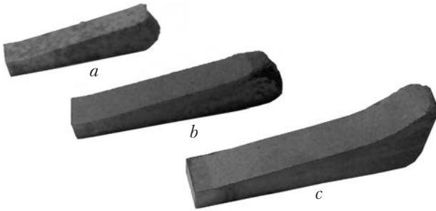
Fig. 3. The view of the samples after the test for compactability: a – mixing; b – mechanosynthesis; c – copperizing
