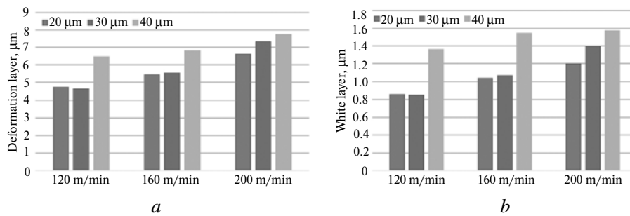
Fig. 9. Effect of the edge radius on the deformation ( a ) and white ( b ) layers.
