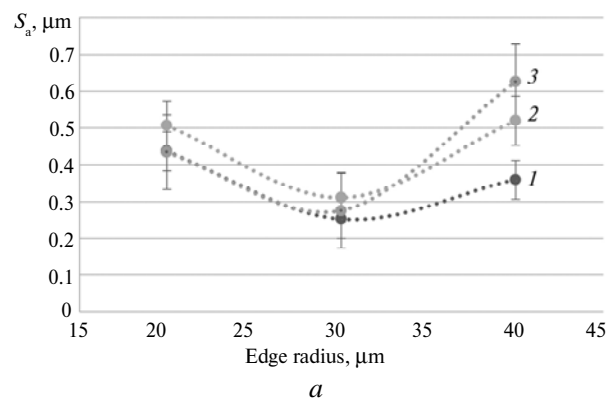
Fig. 5. Effect of edge radius on the surface roughness: 120 (1), 160 (2), 200 (3) m/min.
