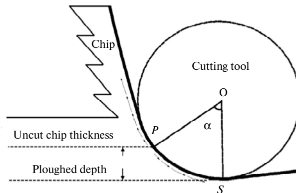
Fig. 1. Schematic view of the shear forces acting on the cutting tool at the stagnation zone.
