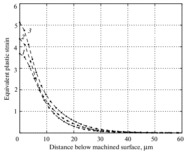
Fig. 7. Equivalent plastic strains in the subsurface for different edge radii: r_{\beta} = 20 (1), 30 (2), 40 (3) \mu\text{m} .
