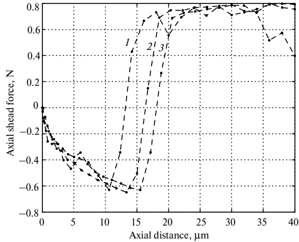
Fig. 3. Axial frictional force component acting on three different edge radii: r_{\beta} = 20 (1), 30 (2), 40 (3) \mu\text{m} .
