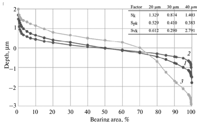
Fig. 6. Abbott-Frestone curves at different turning parameters: 20 (1), 30 (2), 40 (3) \mu\text{m} and 160 m/min.
