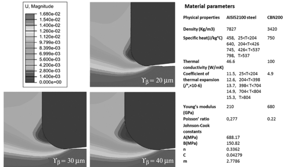
Fig. 2. The material flow of workpiece at three different edges radii.
