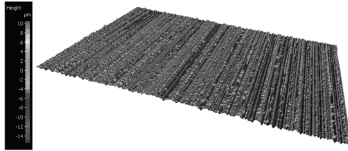
Fig. 4. Typical surface topography measured by Alicona microscope; cutting parameters: \gamma_\beta = 20 \mu\text{m} , v_c = 160 \text{ m/min} , f = 0.08 \text{ mm/rev} , a_p = 0.1 \text{ mm} .
