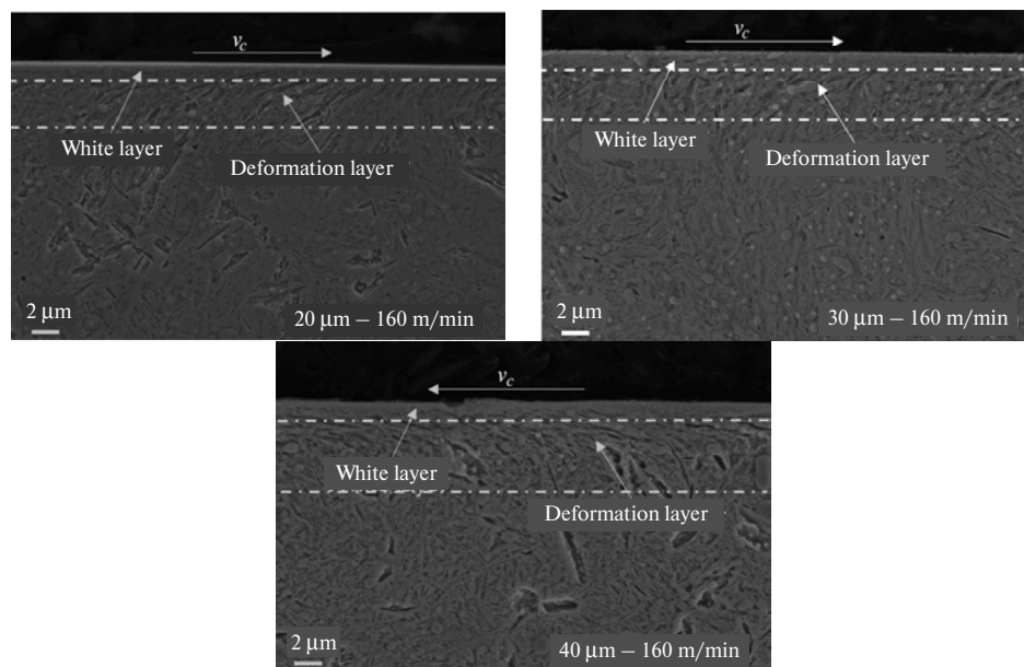
Fig. 8. SEM surface structure at cutting parameters: v_c = 160 m/min, f = 0.08 mm/ref, a_p = 0.1 mm; dry cut; workpiece material – AISI 52100; cutting tool – cBN200.
