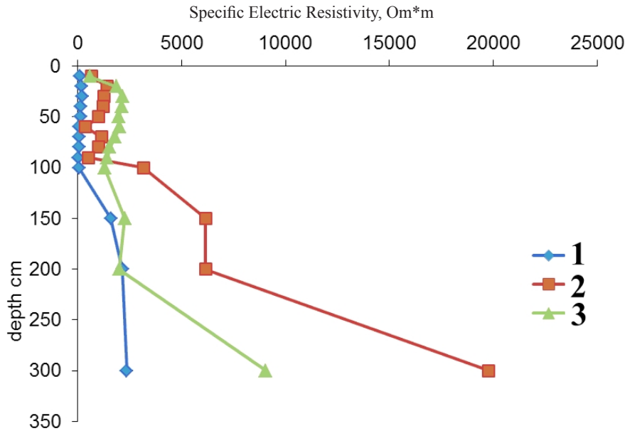
Fig. 2. The vertical electrical resistivity for Point Thomas oasis study sites, Specific Electric Resistivity, Om*m
