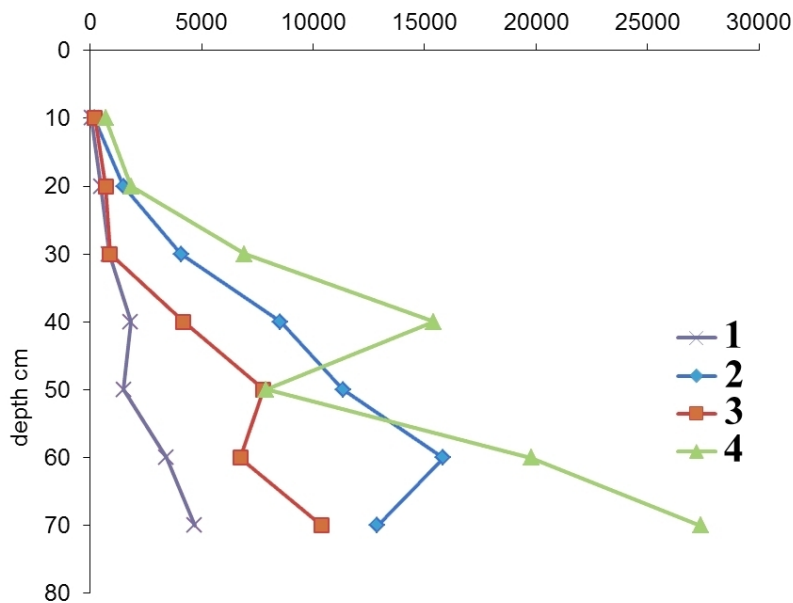
Fig. 1. The vertical electrical resistivity sounding results for Argentine Islands study sites,
