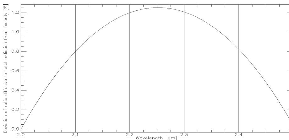
Fig. 2. Deviation of the ratio between diffusive and total radiation from linearity
