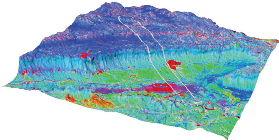
Fig. 1. Case study region Makhtesh Ramon here figured as hill shaded 3D false colour composite that is grey overlaid by the extent of the hyperspectral AISA DUAL acquisition (RGB = Landsat TM (GSD 30 m) mineral ratios 5/7 (clays), 5/4 (FeDEM (is a product of METI and NASA, GSD 15 m))
