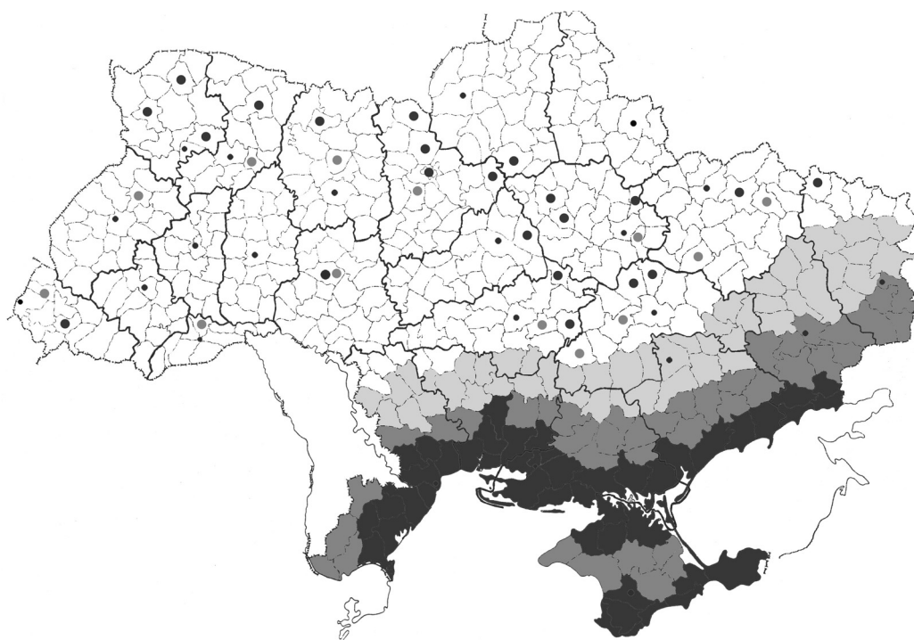
Fig. 1. Natural habitat of Hyalomma marginatum in Ukraine.
