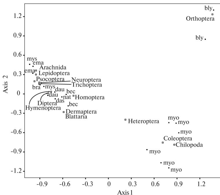
Fig. 3. Correspondence analysis of dietary preferences of the studied Myotis species. Species acronyms as in table 1.
