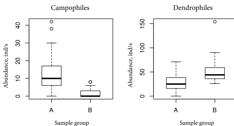
Fig. 3. The abundance (the mean number of individuals per sample) of campophilous and dendrophilous birds in groups of samples A (Clusters I–IV) and B (Clusters V–VI).
