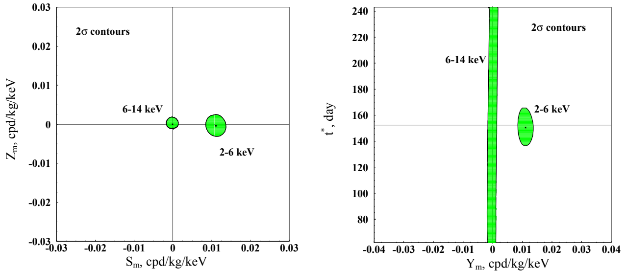
Fig. 4. 2\sigma contours in the plane (S_m, Z_m) (left) and in the plane (Y_m, t^*) (right) for the (2 - 6) keV and (6 - 14) keV energy intervals. The contours have been obtained by the maximum likelihood method, considering the cumulative exposure of 1.17 t \cdot \text{yr} . A modulation amplitude is present in the lower energy intervals and the phase agrees with that expected for DM induced signals. See Refs. [13, 14] and text. (Color Figure online).
