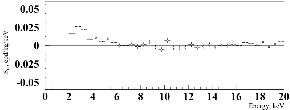
Fig. 3. Energy distribution of the modulation amplitudes S_m for the total cumulative exposure 1.17 \text{ t} \cdot \text{yr} obtained by maximum likelihood analysis. The energy bin is 0.5 keV. A clear modulation is present in the lowest energy region, while S_m values compatible with zero are present just above. In fact, the S_m values in the (6 - 20) keV energy interval have random fluctuations around zero with \chi^2 equal to 27.5 for 28 degrees of freedom. See Refs. [13, 14] and text.
