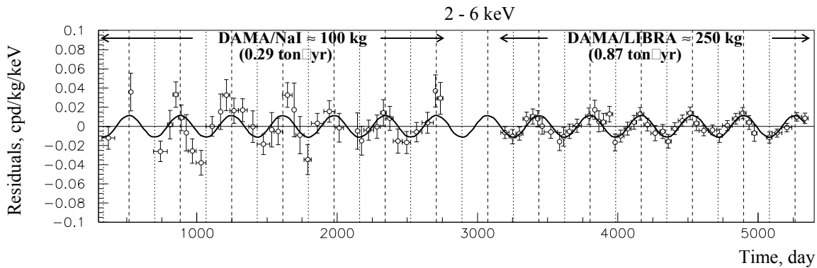
Fig. 1. Experimental model-independent residual rate of the single-hit scintillation events, measured by DAMA/NaI over seven and by DAMA/LIBRA over six annual cycles in the (2 - 6) keV energy interval as a function of the time [4, 5, 13, 14]. The zero of the time scale is January 1 st of the first year of data taking. The experimental points present the errors as vertical bars and the associated time bin width as horizontal bars. The superimposed curve is A \cos \omega(t - t_0) with period T = 2\pi/\omega = 1 yr, phase t_0 = 152.5 day (June 2 nd ) and modulation amplitude, A , equal to the central value obtained by best fit over the whole data: cumulative exposure is 1.17 \text{ t} \cdot \text{yr} . The dashed vertical lines correspond to the maximum expected for the DM signal (June 2 nd ), while the dotted vertical lines correspond to the minimum. See Refs. [13, 14] and text.
