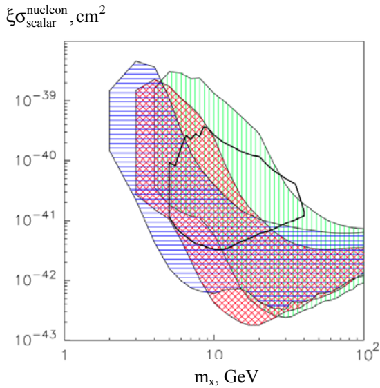
Fig. 5. Regions in the nucleon cross section vs DM particle mass plane allowed by DAMA in three different instances for the Na and I quenching factors: i) without including the channeling effect [(green) vertically-hatched region], ii) by including the channeling effect [(blue) horizontally-hatched region]), and iii) without the channeling effect using the energy-dependent Na and I quenching factors [27] [(red) cross-hatched region]. The velocity distributions and the same uncertainties as in Refs. [4, 5] are considered here. The allowed region obtained for the CoGeNT experiment, including the same astrophysical models as in Refs. [4, 5] and assuming for simplicity a fixed value for the Ge quenching factor and a Helm form factor with fixed parameters, is also reported and denoted by a (black) thick solid line. For details see Ref. [27]. (Color Figure online).
