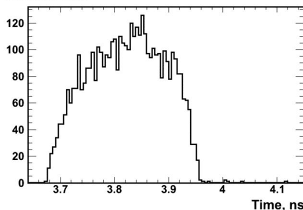
Fig. 4. LEETECH timing characteristics for “wide” mode of collimator system (simulation).
