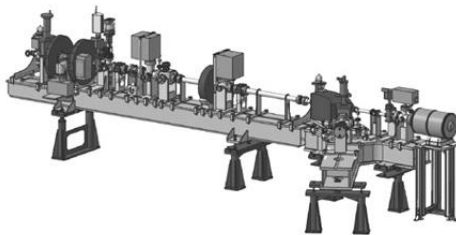
Fig. 1. General view of PHIL photoinjector.
