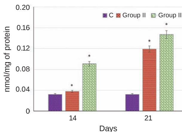
Fig. 5. The content of Schiff bases in the mitochondrial fraction of rat liver under the influence of diethyl phthalate: C – intact animals (control); Group II – rats administered diethyl phthalate at a dose of 2.5 mg/kg; Group III – rats administered diethyl phthalate at a dose of 5.4 mg/kg; *statistically significant difference compared to the control group, P < 0.05
