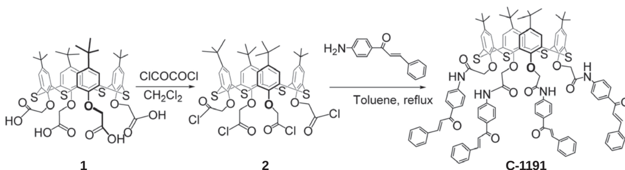
Fig. 2. Synthesis of 5,11,17,23-tetra- tert -butyl-25,26,27,28-tetra[(4'-benzylideneacetophenonyl)aminocarbonylmethoxy]-thiacalix[4]arene C-1191 ( cone )
