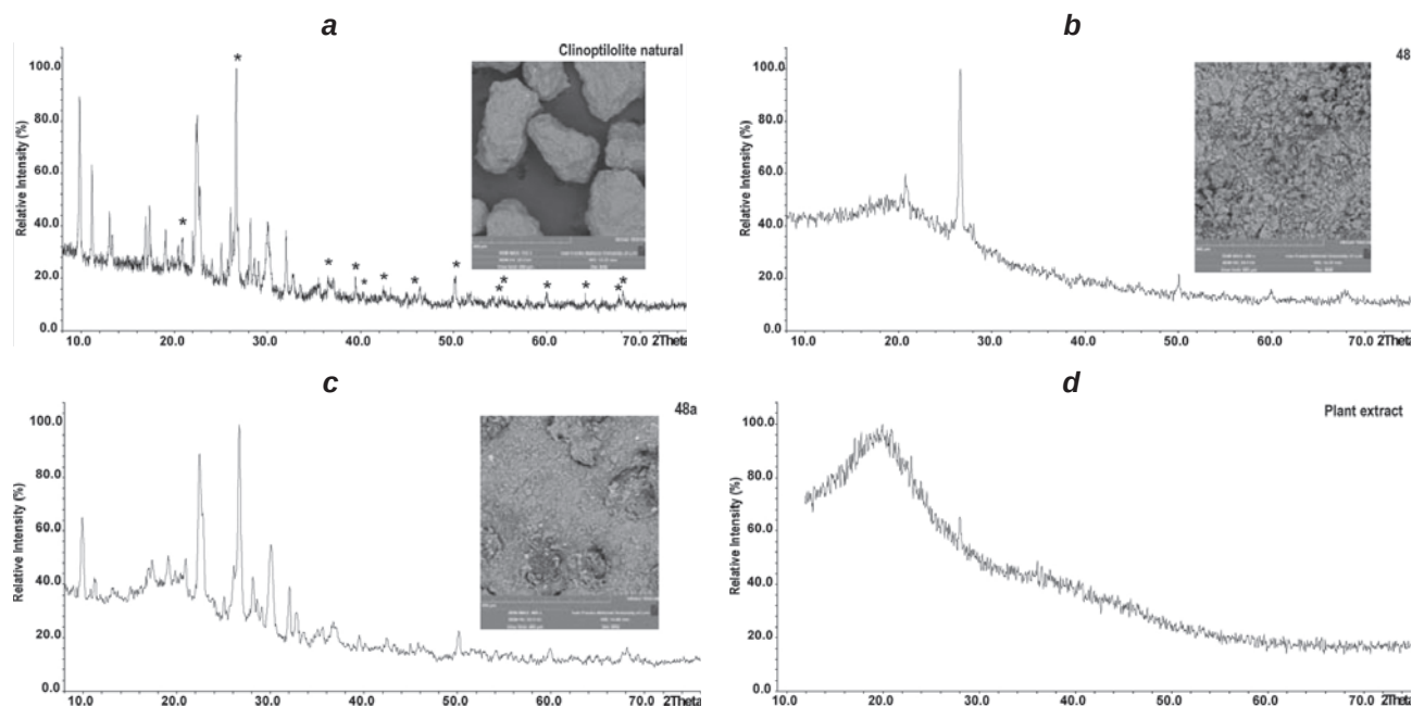
Fig. 1. Diffraction pattern of natural CL (a), the samples after milling with plant extract in air (b – No. 48), and ethanol medium (c – No. 48a). Asterisks indicate the peaks from the concomitant \alpha -quartz phase. On the insert SEM images of the corresponding samples. Diffraction pattern of plant extract (d)
