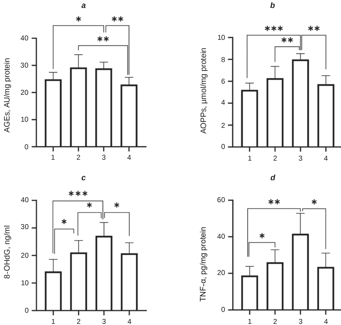
Fig. 2. Levels of AGEs (a), AOPPs (b), 8-OHdG (c) and TNF- \alpha (d) in the brain homogenates. Data are presented as mean \pm SD. * P < 0.05 , ** P < 0.01 , *** P < 0.001
