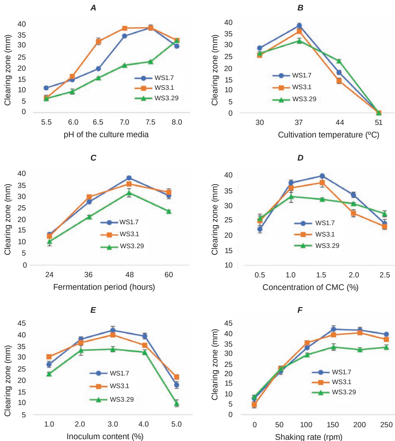
Fig. 6. Effects of different factors on the cellulolytic activity of three selected bacterial strains. A – Effect of pH; B – effect of temperature; C – effect of incubation time; D – effect of CMC substrate concentration; E – effect of inoculum content; F – effect of shaking rate
