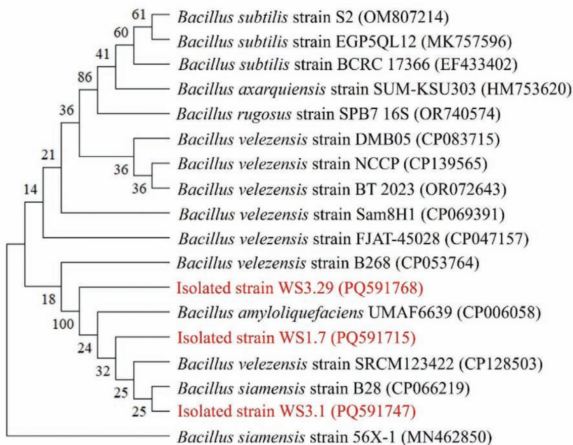
Fig. 5. Phylogenetic analysis of the the WS1.7, WS3.1 and WS3.29 isolates
