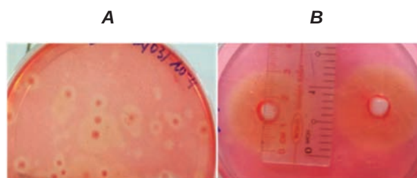
Fig. 1. CMC hydrolysis zones of colonies (A) and of crude enzyme (B)
