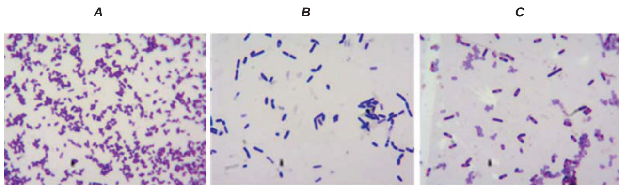
Fig. 3. Gram test results for the WS1.7 (A), WS3.1 (B), and WS3.29 (C) isolates
