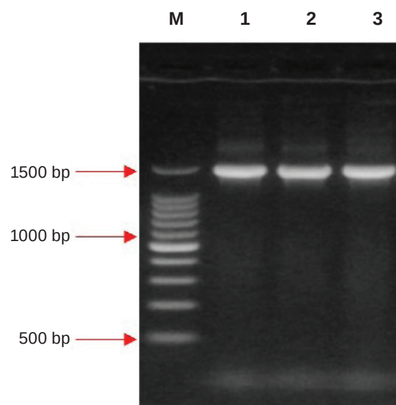
Fig. 4. Agarose gel electrophoresis of PCR amplified products of the 16S rRNA gene. Lane M – Marker; Lane 1 – WS1.7; Lane 2 – WS3.1; Lane 3 – WS3.29
