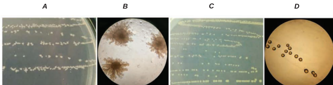
Fig. 2. WS3.9 (A, B) and WS1.18 (C, D) isolate colonies on CMC-agar media
