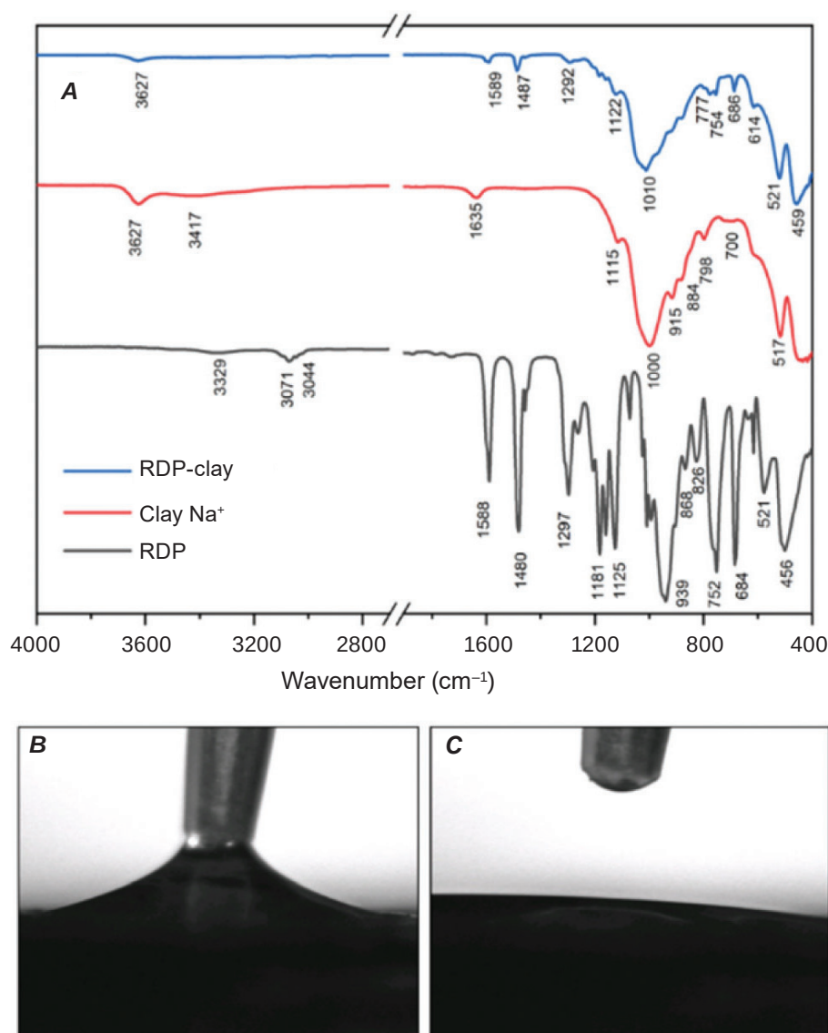
Fig. 3. Profile of RDP-clay compared to just RDP and pure sodium clay captured using FTIR to show the chemical bonds and functional groups present in individual RDP-clay particles. Images represent 100% RDP-clay surfaces tested with water contact angle image analysis using an optical contact angle meter before (B) and after (C) applying 5 \mu\text{l} of water
