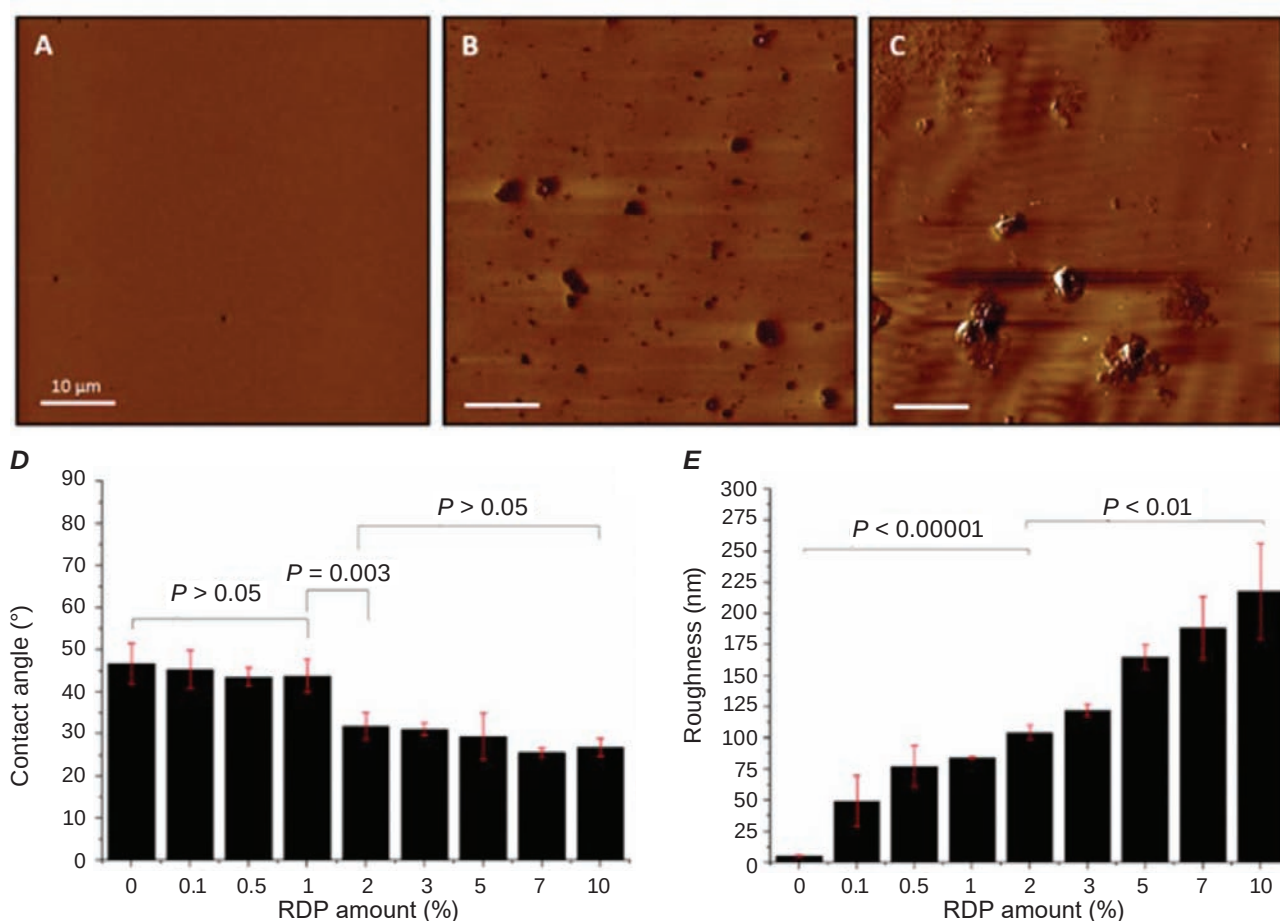
Fig. 4. Images of PVA/RDP surfaces using AFM scans. Friction images of 50 \mu\text{m}^2 are shown for RDP-clay inclusions (A) Control, (B) 2%, and (C) 10% with white ( 10 \mu\text{m} ) magnification bars. Color ranges for z-scale of images are 0–190 nm. PVA/RDP-clay thin film surfaces were studied by (D) water contact angle analysis and (E) surface roughness quantification. Bar graphs represent mean \pm SEM
