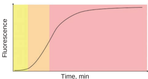
Fig. 1. The change in the fluorescent signal over time, reflecting the generation of thrombin in blood plasma, which is initiated by tissue factor and \text{CaCl}_2 (yellow – initiation phase, orange – amplification phase, and resulting phase) [1] with permission
