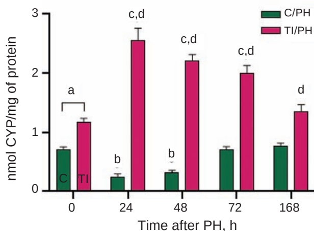
Fig. 3. Cytochrome P450 content in the microsomal fraction of the livers of rats under conditions of partial hepatectomy following acetaminophen-induced toxic injury. C/PH – control animals that underwent partial hepatectomy; TI/PH – rats that underwent partial liver resection after acute acetaminophen-induced toxic injury. a, b, c – values indicated by these letter indices differ statistically significantly; a – statistically significant difference between the TI group and the control group (C) at 0 h; b – statistically significant difference of the C/PH groups compared to the C group at 0 h; c – statistically significant difference of the TI/PH groups compared to the TI group at 0 h; d – statistically significant difference of the TI/PH groups compared to the C/PH groups
