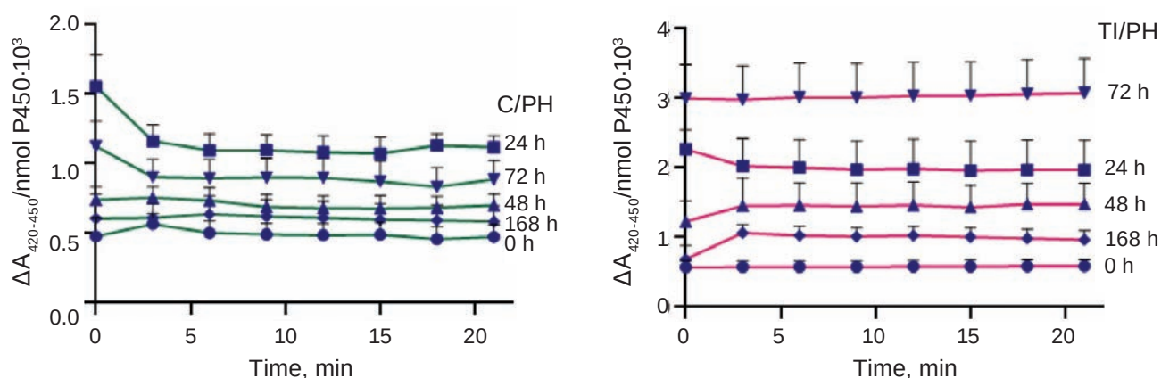
Fig. 4. The rate of cytochrome P450 inactivation in the microsomal fraction of the livers of rats under conditions of partial hepatectomy following acetaminophen-induced toxic injury
