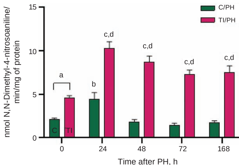
Fig. 2. N-oxygenase activity of cytochrome P450 in the microsomal fraction of the livers of rats under conditions of partial hepatectomy following acetaminophen-induced toxic injury. C/PH – control animals that underwent partial hepatectomy; TI/PH – rats that underwent partial liver resection after acute acetaminophen-induced toxic injury. a, b, c – values indicated by these letter indices differ statistically significantly; a – statistically significant difference between the TI group and the control group (C) at 0 h; b – statistically significant difference of the C/PH groups compared to the C group at 0 h; c – statistically significant difference of the TI/PH groups compared to the TI group at 0 h; d – statistically significant difference of the TI/PH groups compared to the C/PH groups
