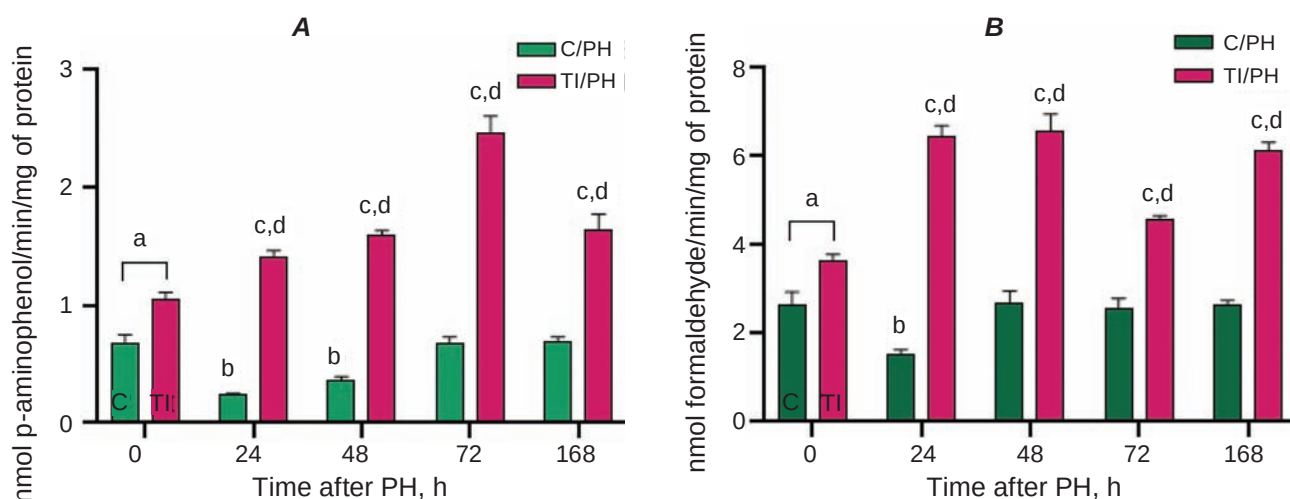
Fig. 1. p -Hydroxylase activity (A) and N -demethylase activity (B) of cytochrome P450 in the microsomal fraction of the livers of rats under conditions of partial hepatectomy following acetaminophen-induced toxic injury. C/PH – control animals that underwent partial hepatectomy; TI/PH – rats that underwent partial liver resection after acute acetaminophen-induced toxic injury. a, b, c – values indicated by these letter indices differ statistically significantly; a – statistically significant difference between the TI group and the control group (C) at 0 h; b – statistically significant difference of the C/PH groups compared to the C group at 0 h; c – statistically significant difference of the TI/PH groups compared to the TI group at 0 h; d – statistically significant difference of the TI/PH groups compared to the C/PH groups
