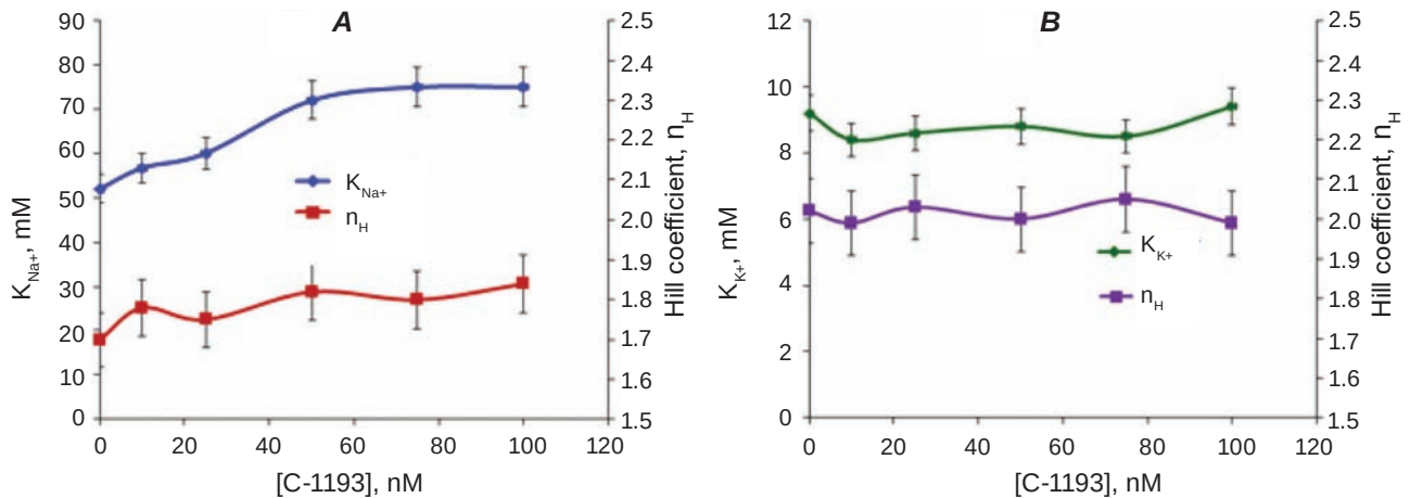
Fig. 4. The action of thiacalix[4]arene C-1193 on the kinetic parameters of the dependence of the activity of Na + ,K + -ATPase in PM fraction of the myometrium cells on the concentration of Na (A) and K (B) ions ( M \pm m , n = 5 )
