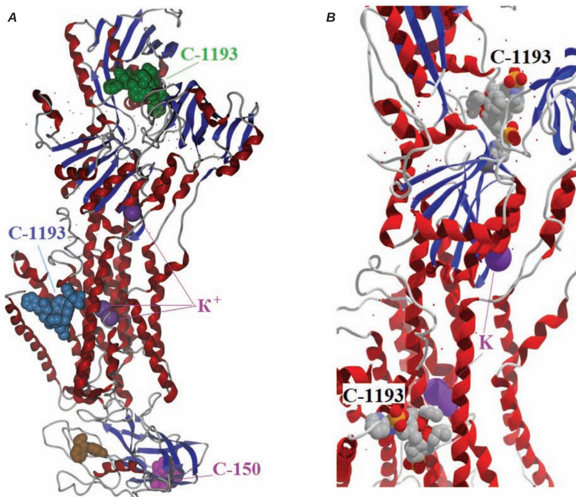
Fig. 7. A – The most probable places of C-1193 binding with active sites of \text{Na}^+/\text{K}^+ -ATPase, obtained by the docking method; B – the position of C-1193 after molecular dynamics of the complex of thiacalix[4]arene and N- and transmembrane domains in the interval of 6 ns/1 ns
