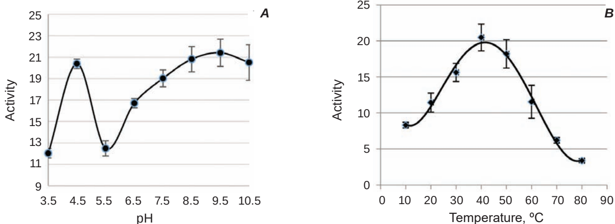
Fig. 3. Enzyme activity at different pH values (A) and temperatures (B): the ordinate axis shows activity ( \mu\text{mol} leucine/mg protein/min), and the abscissa axis indicates pH values (A) and temperature in °C (B)
