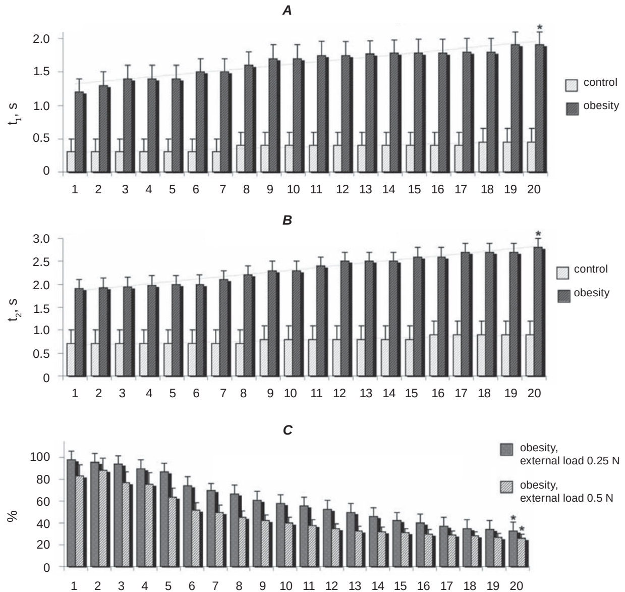
Fig. 3. Time required for musculus soleus contraction to return to the initial state (A – t_1 ; B – t_2 ) and maximum contraction force expressed as a percentage of the control value (C) after non-relaxation stimulation at 50 Hz for 6 s with external loads of 0.25 and 0.5 N. Numbers 1-20 correspond to consecutive muscle contractions. * P < 0.05 , significant difference compared with the Control group
