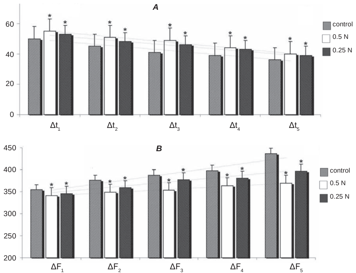
Fig. 5. Time intervals ( \Delta t_1 - \Delta t_5 , ms) between maximal force responses of musculus soleus (A) and amplitudes of musculus soleus contractions ( \Delta F_1 - \Delta F_5 , mN) (B) during five sequential contractions forming incomplete (unfused) tetanus at 20 Hz stimulation. Control – control animals; 0.25 and 0.5 N – external loads of 0.25 and 0.5 N, respectively. * P < 0.05 , significant difference compared with the Control group
