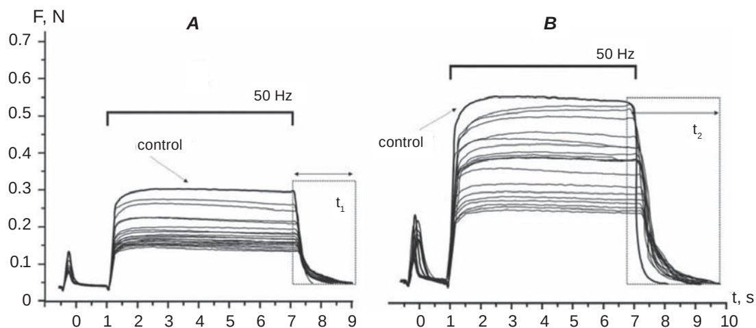
Fig. 2. Musculus soleus mechanograms of a representative experimental animal from the Obesity group recorded during 20 consecutive non-relaxation electrostimulation signals at 50 Hz. Averaging was performed for 10-15 obtained force curves. Under the same conditions, no significant changes in the strength response were observed in control animals. A – external load 0.5 N; B – external load 0.25 N; control – contraction of musculus soleus in control animals; t_1 , t_2 – time intervals representing the period required for the muscle to return to baseline tension after termination of stimulation
