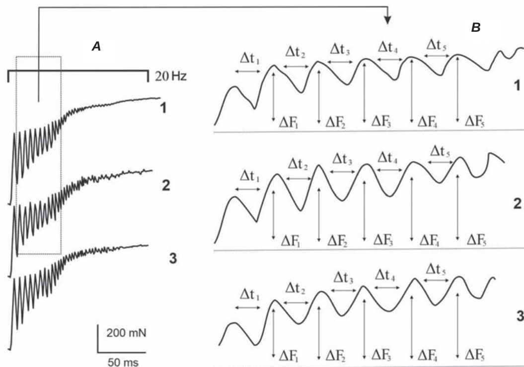
Fig. 4. Typical curve of the musculus soleus contractile response to stimulation with impulses applied at 20 Hz for 6 s (A); development of incomplete tetanus during the first five peaks of the musculus soleus force response to 20 Hz stimulation in obese rats (B). 1 – contraction curves recorded in control animals; 2 – external load 0.25 N; 3 – external load 0.5 N; \Delta t_1 - \Delta t_5 – time intervals between sequential contraction peaks; \Delta F_1 - \Delta F_5 – amplitude of force generated during sequential contractions of musculus soleus
