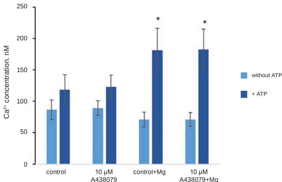
Fig. 6. A438079 effects on [Ca^{2+}]_i . Means \pm SEM; n = 4 . P < 0.05 compared to the probe without Mg^{2+}
