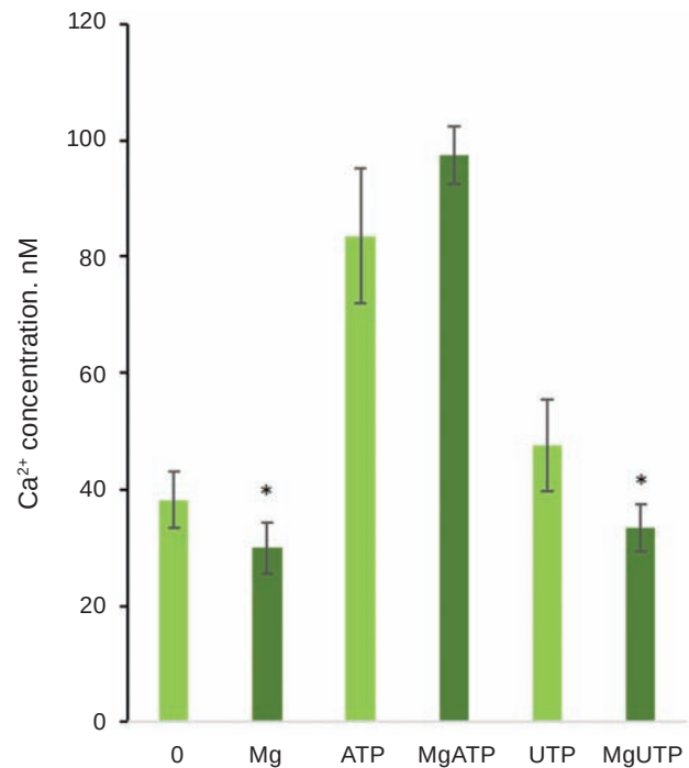
Fig. 5 Comparison of the ATP and UTP effects [Ca^{2+}]_b . Means \pm SEM; n = 6 . P < 0.05 compared to the probe without Mg^{2+}
