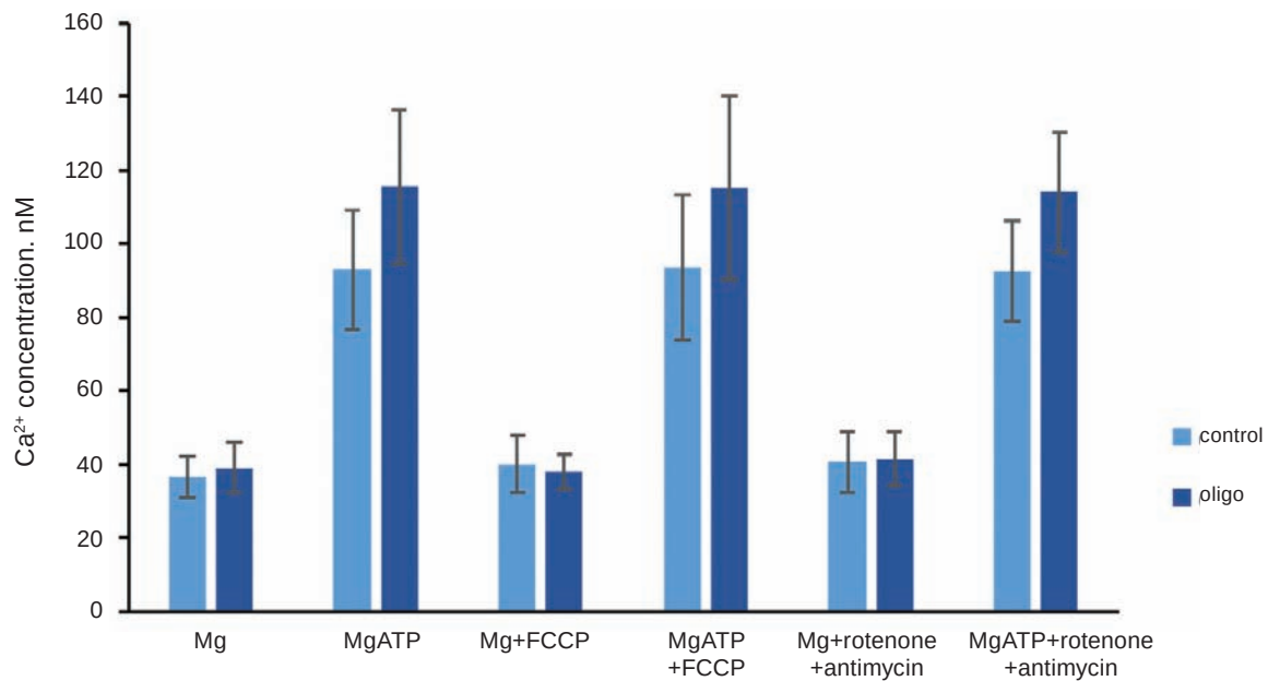
Fig. 2. [Ca^{2+}]_b upon activation (1 \mu M FCCP) or inhibition (1 \mu M rotenone + 2 \mu g/ml antimycin A) of the respiratory chain. Testing was carried out in the absence (control) or presence of 1 \mu g/ml oligomycin (oligo). Means \pm SEM, n = 4
