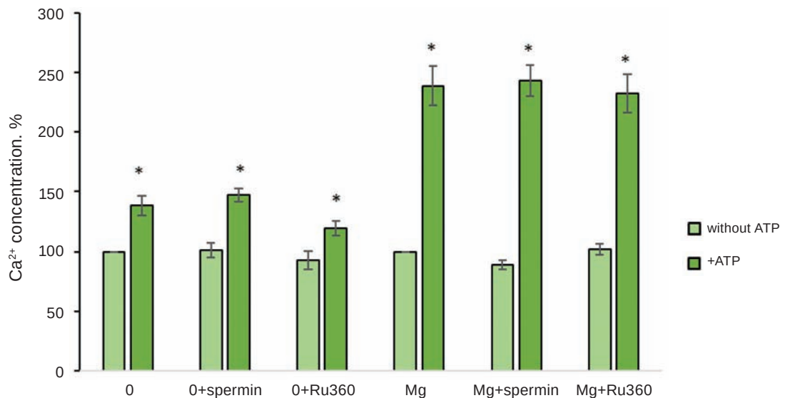
Fig. 3. [Ca^{2+}]_b at activation (1 mM spermine) or inhibition (10 \mu M Ru360) of the Ca^{2+} uniporter. Means \pm SEM, n = 4 , P < 0.05 compared to the probe without ATP
