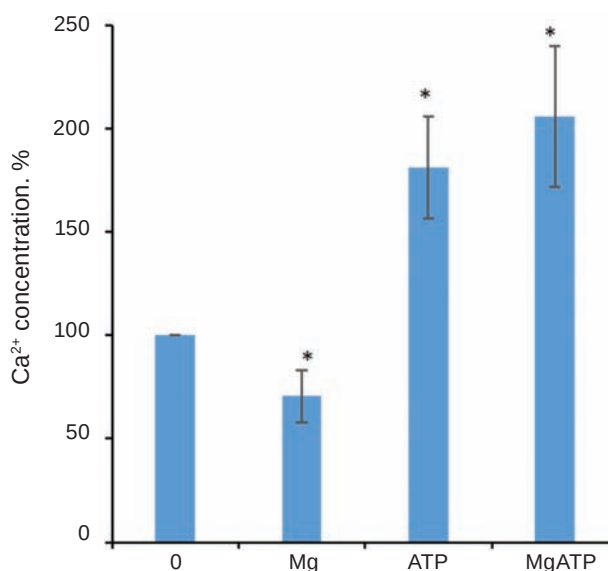
Fig. 1. Effects of 3 mM Mg 2+ , 3 mM ATP or 3 mM Mg 2+ ATP on [Ca^{2+}]_b . The [Ca^{2+}]_b was measured in a medium containing: 250 mM sucrose, 2 mM K + -phosphate buffer, 5 mM sodium succinate, ±3 mM MgCl 2 , ±3 mM ATP, 20 mM Hepes, pH 7.4. The calibration of the Fluo-4 fluorescence was performed at the end of each testing probe by adding 0.1% Triton X-100 (in the presence of 100 µM CaCl 2 ) and, in 1 min, 5 mM EGTA (fluorescence intensities F_{max} and F_{min} , respectively). Calculations using the Grynkiewicz equation were performed at the end of 10 min of incubation (using the average value of the last 10 data points). Means ± SEM, n = 5, P < 0.05 compared to control
