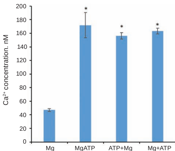
Fig. 4. [Ca^{2+}]_b and the time of Mg^{2+} or ATP addition: Mg – 3 mM Mg^{2+} was added at the start of testing, incubation 10 min; MgATP – 3 mM Mg^{2+} ATP was added at the start of testing, incubation 10 min; ATP+Mg – 3 mM ATP was added at the start of testing, incubation 5 min followed by 3 mM Mg^{2+} addition and next 5 min incubation; Mg+ATP – 3 mM Mg^{2+} was added at the start of testing, incubation 5 min followed by 3 mM ATP addition and next 5 min incubation. Baseline Ca^{2+} concentration was calculated at the end of 10 min incubation. Means \pm SEM, n = 4 , P < 0.05 compared to control (Mg)
