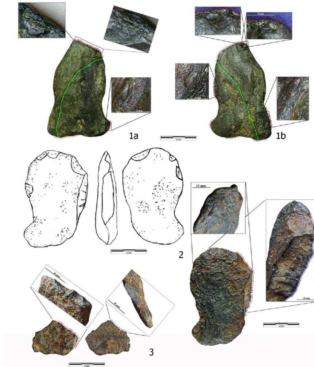
Fig. 2. Medzhibozh 1, artefacts with post-depositional alterations. Refitted flint pebble (1), chopper on flint pebble (2), flint flake with retouched and trimmed edges from layer IV (3). Numbers 1 and 2 demonstrate cracks and pits, and numbers 2 and 3 show scars of different states of preservation. Red dots point to artificial damage; blue dots point to post-depositional alterations; green line marks a border between joining fragments. Database IDs: 1 – MJ/1/09/16b/96, 2 – MJ1/09/16b/30, 3 – MJ1/00/IV/27
