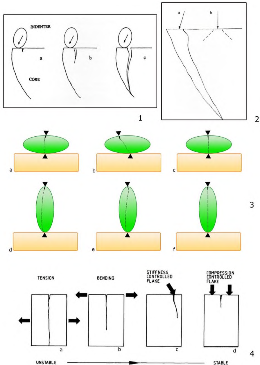
Fig. 7. Some basic features of a flake detachment process. 1. Scheme of crack propagation: initiation (a), propagation (b), termination (c) after Odell [2004, fig. 3.1.]. 2. Flake detachment through Herzian fracture near the edge of core (a) and far from the edge (b), after Odell [2004, fig. 3.7.]. 3. Scheme of some variations of bipolar-on-anvil knapping, a–f, after van der Drift [2009, fig. 5]. 4. The stability of crack propagation is higher in the case of bipolar knapping (d) after Cotterell & Kamminga [1987, fig. 16]
