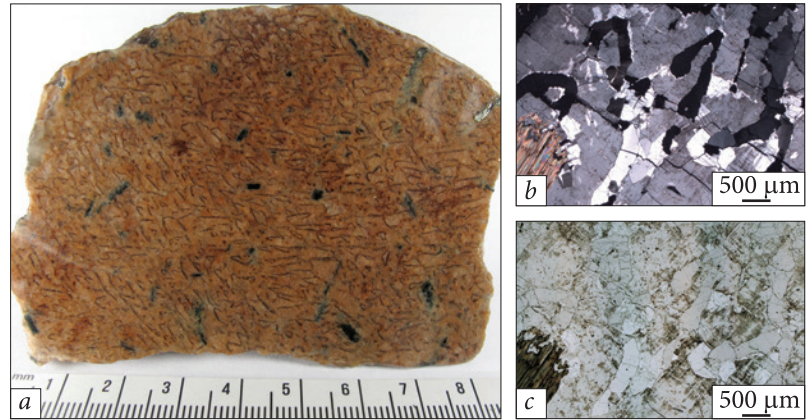
Fig. 3. Fragment of vein of aplite-pegmatoid granite, sample 21/23, pegmatite: a — general view; b — pegmatite structure of intergrowth of potassium feldspar (gray grains) with quartz (white and dark vermiform grains) and with cracks filled with albite (light rectangular grains with polysynthetic twins) optical microscope Carl Zeiss Axio Imager 2 for materials, the analyzer is introduced; c — too, without an analyzer
