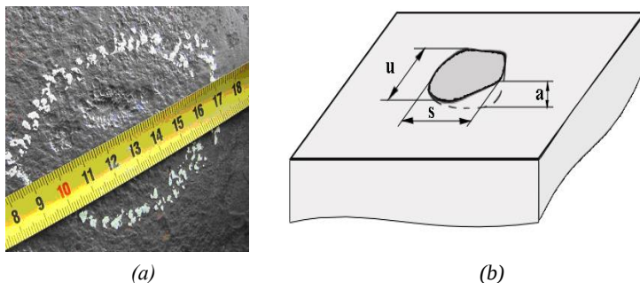
Fig. 1. Appearance (a) and schematic representation (b) of a typical defect of local corrosion loss of metal
