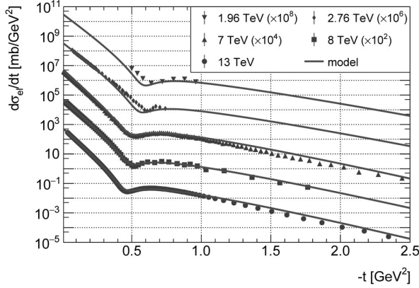
Fig. 6. Elastic pp differential cross section data described by a dipole Regge exchange model with both pomeron and odderon contributions
