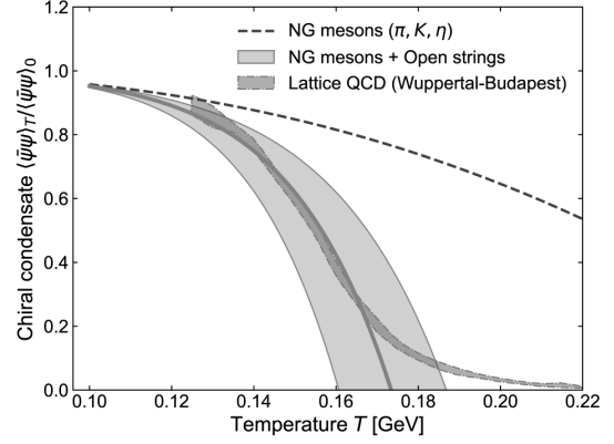
Fig. 5. Ratio of the chiral condensate at finite temperature to its value at zero temperature. The lattice data are taken from Ref. [18]. Figure taken from Ref. [1]
