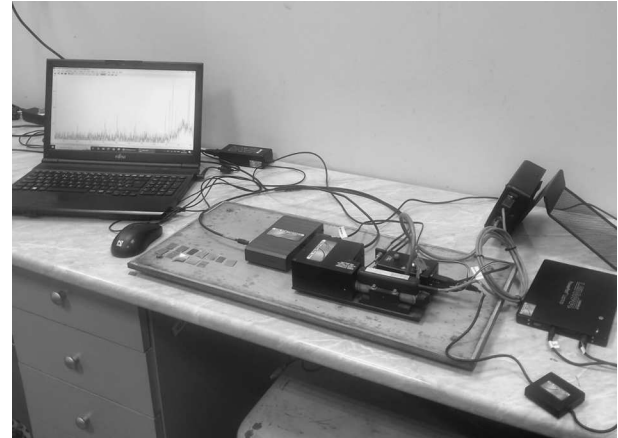
Fig. 1. StellarNet Blue-Wave (200–400 nm) spectroscopic system for LIBS and absorption measurements: laser–target interaction, optical fiber collection, and spectrometer-based detection
