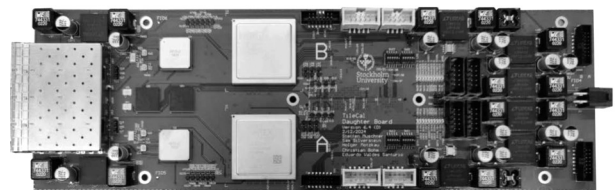
Fig. 6. Daughterboard
