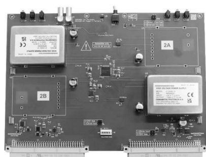
Fig. 9. HVPS Board
