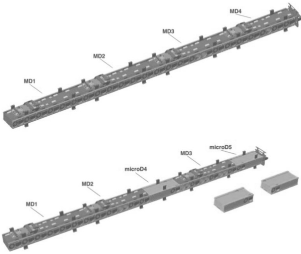
Fig. 2. TileCal Mechanics
