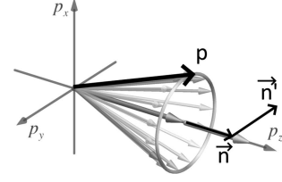
Fig. 3. Momentum space illustration of the vortex neutron: the cone represents the plane-wave components with momenta \mathbf{p} , which are not parallel to the average propagation direction \mathbf{n} . The scattered neutron moves along \mathbf{n}'
