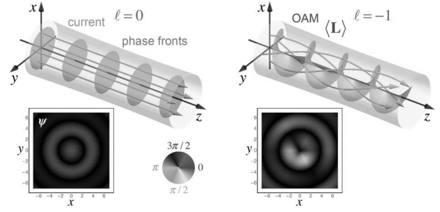
Fig. 1. The current lines and phase fronts of non-vortex Gaussian state (left) and an \ell = -1 vortex state (right). The insets show the intensity distributions in the transverse plane as well as the phase encoded in color. Adapted from [1]
