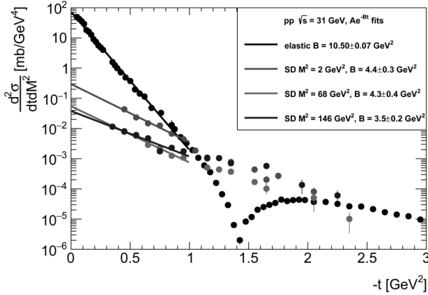
Fig. 12. Elastic pp scattering and single-diffractive dissociation differential cross section data at \sqrt{s} = 31 GeV as a function of -t
