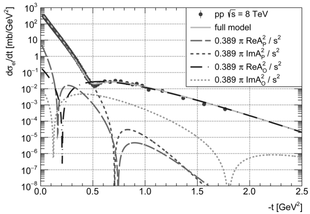
Fig. 8. Contribution of the real and imaginary parts of the pomeron and odderon components of the amplitude to the description of the pp differential cross section data at \sqrt{s} = 8 TeV
