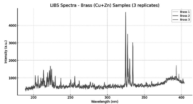
Fig. 4. Spectral profiles of the three replicates of brass
