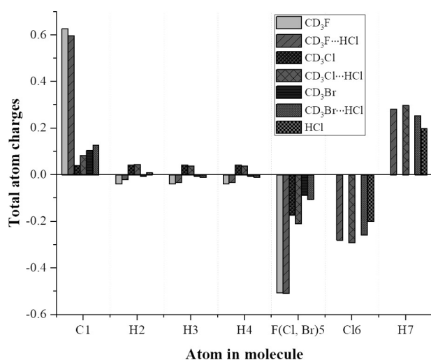
Fig. 4. Schematic representation of the total atomic charge distribution for the studied complexes
