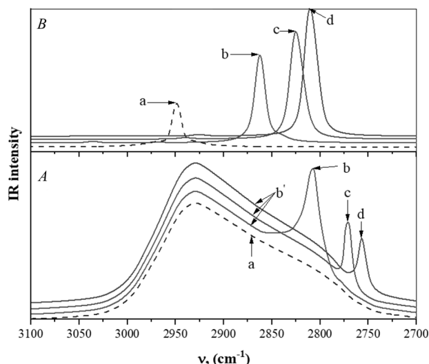
Fig. 1. Absorption spectra of the \nu(\text{HCl}) stretching band in argon at 120 K (A): (a) free HCl, (b) HCl + \text{CD}_3\text{F} , (c) HCl + \text{CD}_3\text{Cl} , and (d) HCl + \text{CD}_3\text{Br} . The sharp bands of the complexes appear on the P-branch side of the free HCl line. Corresponding spectra calculated using anharmonic vibrational frequency approximations (B)
