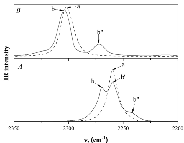
Fig. 3. Absorption spectra (A) of the \nu_{\text{ass}}(\text{CD}_3) stretching band in liquid argon: (a) free \text{CD}_3\text{F} , (b) \text{CD}_3\text{F} + \text{HCl} mixture, (b') free \text{CD}_3\text{F} molecules present in the mixture, and (b'') overtone band of the \nu_{\beta}(\text{CD}_3) vibration. Calculated spectra (B) obtained using anharmonic frequency approximations, confirming the assignment of the b'' band to the \nu_{\beta}(\text{CD}_3) overtone
