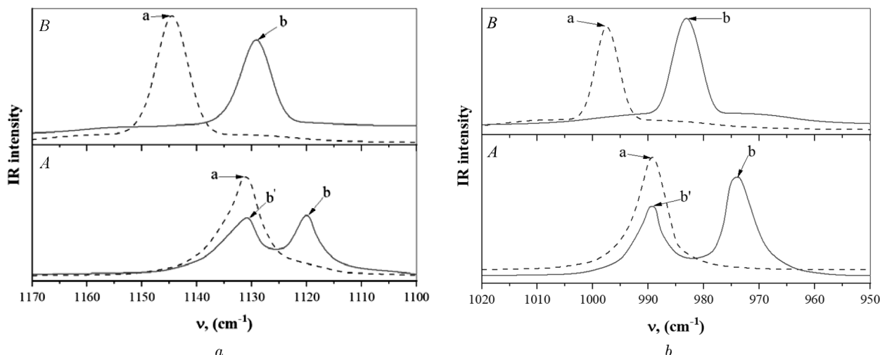
Fig. 2. Absorption spectra (A) of CD_3F (a) and a CD_3F + HCl mixture (b) in liquid argon. Calculated spectra (B) using anharmonic approximations. Vibrational assignments: \nu_\beta(CD_3) (left) and \nu(CF) (right)
