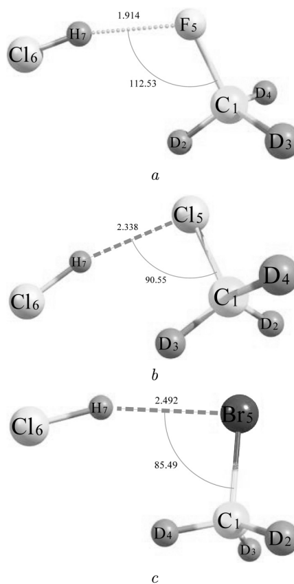
Fig. 5. Optimized geometries of the CD_3F \cdots HCl , CD_3Cl \cdots HCl , and CD_3Br \cdots HCl complexes calculated at the MP2/6-311++G(3df,3pd) level. Intermolecular features are highlighted, with hydrogen bond lengths and key angles indicated
