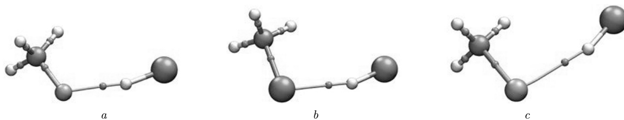
Fig. 6. Bond critical points (BCPs) in the complexes: \text{CD}_3\text{F}\cdots\text{HCl} (a), \text{CD}_3\text{Cl}\cdots\text{HCl} (b), and \text{CD}_3\text{Br}\cdots\text{HCl} (c), obtained from AIM topological analysis
