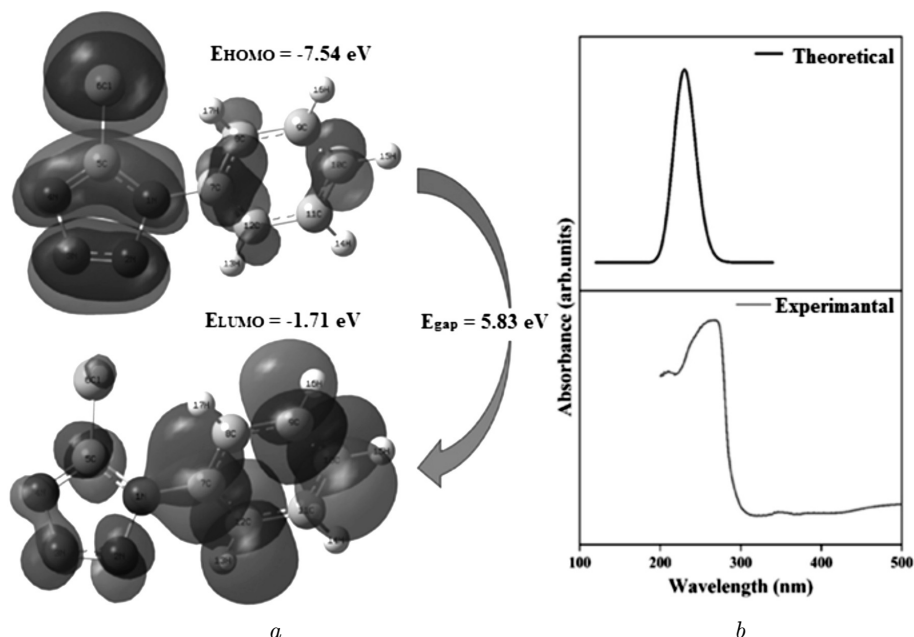
Fig. 4. HOMO-LUMO (a) and UV-Vis spectrum of 5-chloro-1-phenyl-1H-tetrazole (b)
