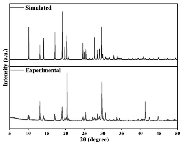
Fig. 2. Simulated and experimental comparison of XRD for 5-chloro-1-phenyl-1H-tetrazole
