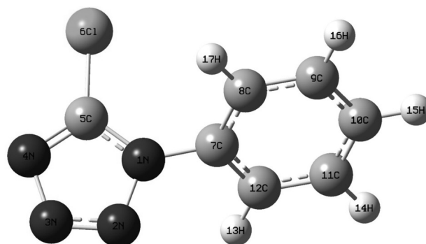
Fig. 1. Optimized structure of 5-chloro-1-phenyl-1H-tetrazole
