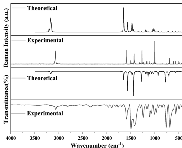
Fig. 3. FT-IR and FT-Raman spectra of 5-chloro-1-phenyl-1H-tetrazole
