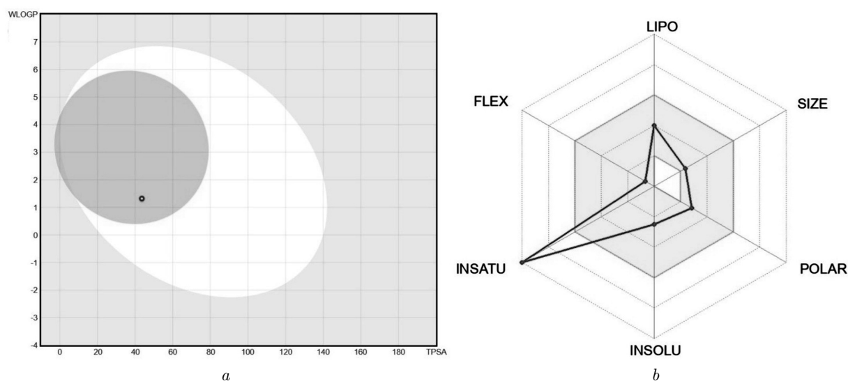
Fig. 8. Boiled Egg and (a) Radar plot of 5-chloro-1-phenyl-1H-tetrazole (b)
