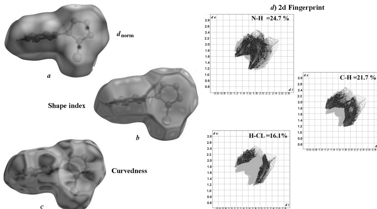
Fig. 6. d_{\text{norm}} (a), Shape index (b), Curvedness (c) and 2D Fingerprint plot of 5-chloro-1-phenyl-1H-tetrazole (d)
