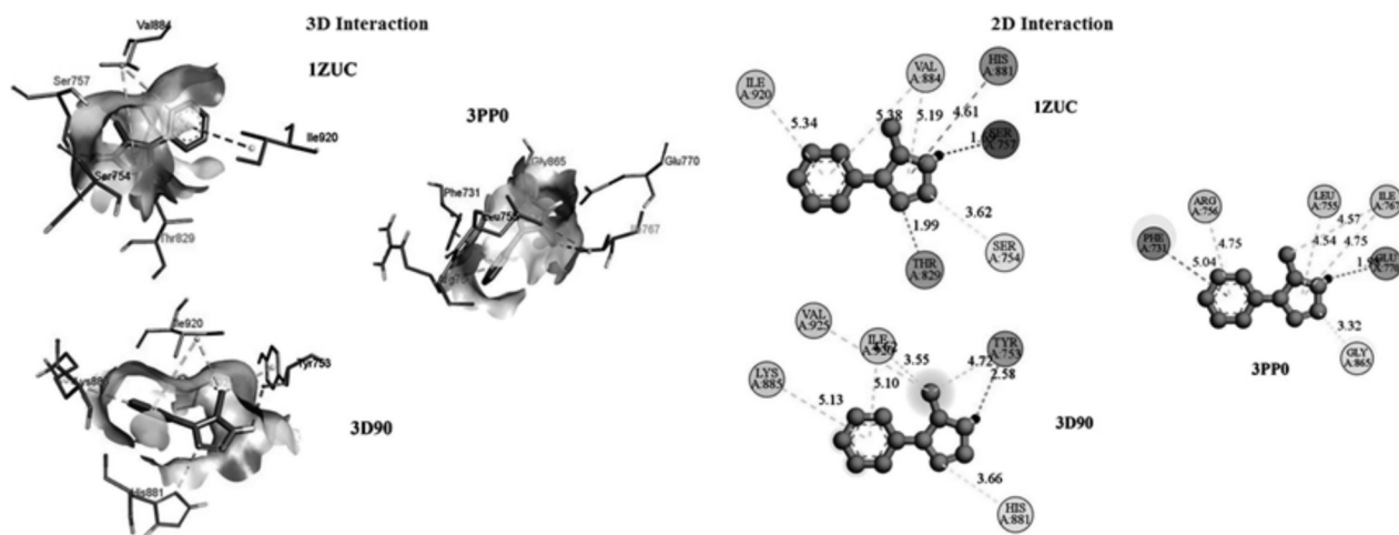
Fig. 7. Molecular docking of 3D and 2D interaction with H-Bond donor-acceptor for 5-chloro-1-phenyl-1H-tetrazole with 1ZUC, 3D90, 3PP0 target proteins
