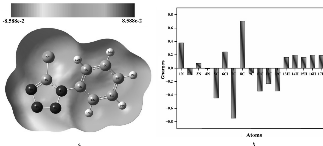
Fig. 5. MEP plot (a) and Mulliken charge analysis of 5-chloro-1-phenyl-1H-tetrazole (b)
