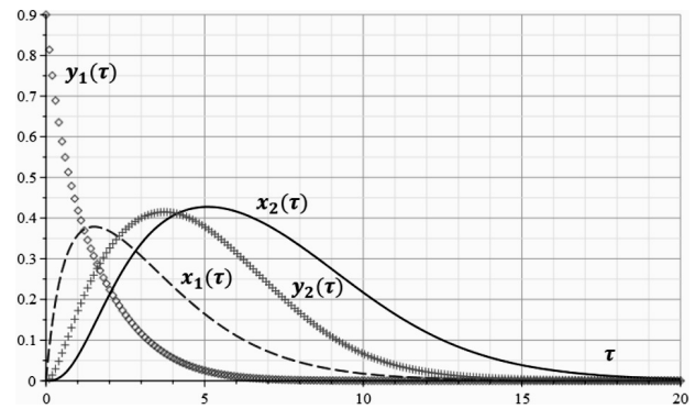
Fig. 3. The same as in Fig. 2, but for \alpha = 0.5 , \beta = 1 , m_0 = 0.9
