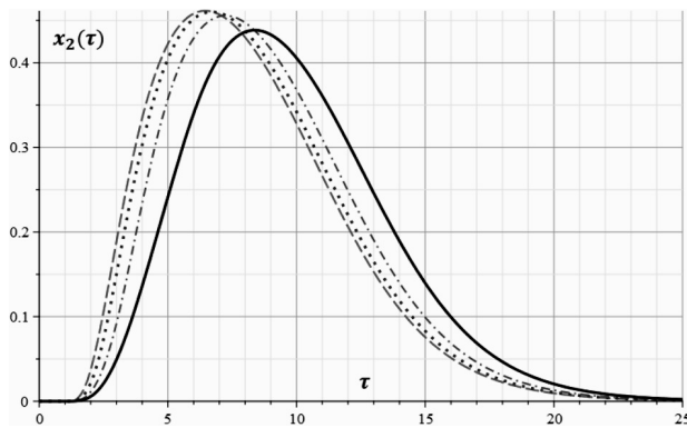
Fig. 6. Dependences of the concentration of activated receptors on the second postsynaptic membrane for various types of input signal at the first synapse (provided that the amount of mediator supplied to the synapse is constant, AT = 1 ): the signal amplitude A = 2 (dashed curve), 1 (dotted curve), 0.5 (dash-dotted curve), and 0.25 (solid curve)
