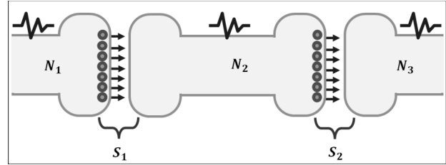
Fig. 1. The system under study: N_1 is the first (input) neuron, N_2 is the second (central) neuron, N_3 is the third (output) neuron, S_1 is the first synapse, S_2 is the second synapse
