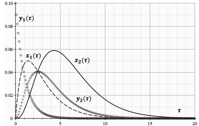
Fig. 2. Time-dependences of the model parameters in the linear approximation: x_1(\tau) (dashed curve), x_2(\tau) (solid curve), y_1(\tau) (diamonds), y_2(\tau) (crosses). \alpha = 0.5 , \beta = 1 , m_0 = 0.1
