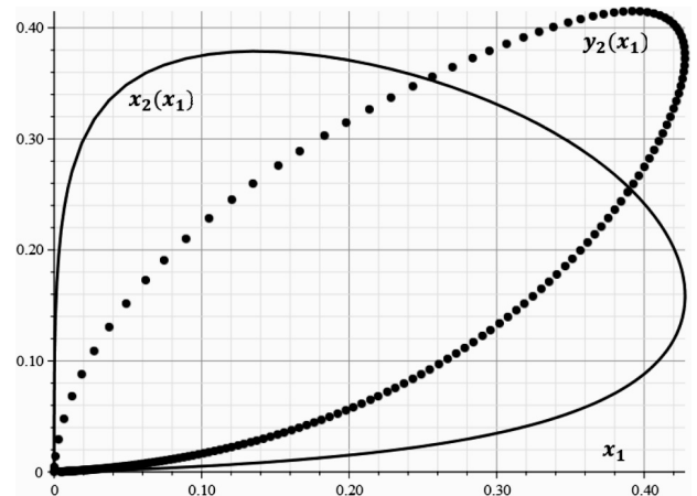
Fig. 4. Phase trajectories of the dependences of the concentration of activated receptors in the second synapse, x_2 (solid curve), and the mediator concentration in the second synapse, y_2 (spheres), on the concentration of activated receptors in the first synapse, x_1 . \alpha = 0.5 , \beta = 1 , m_0 = 0.9
