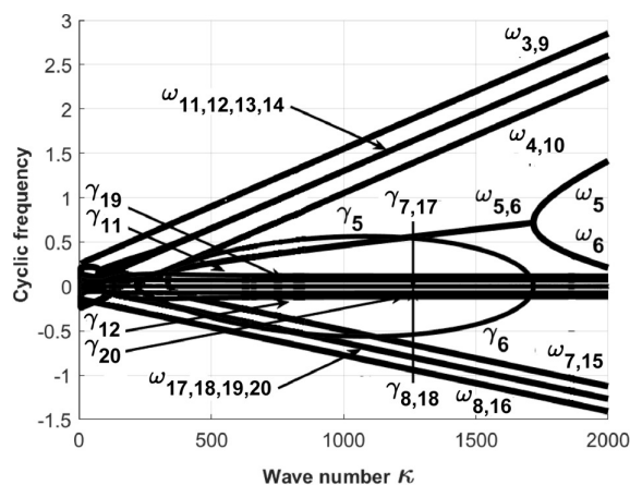
Fig. 12. The same as in Fig. 9, but at \theta = 60^\circ
