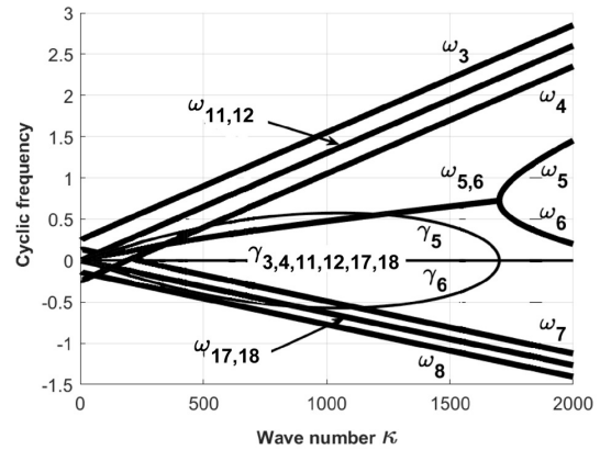
Fig. 9. Dispersion branches of hybrid plasmon-polaritons at \theta = 0^\circ
