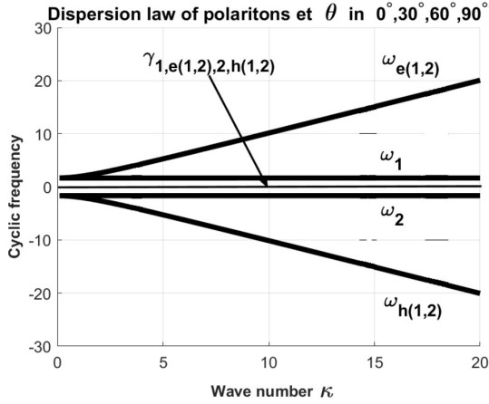
Fig. 6. Dispersion branches of ordinary plasmons and plasmon-polaritons at \theta = 0^\circ, 30^\circ, 60^\circ , and 90^\circ
