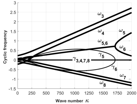
Fig. 4. The same as in Fig. 2, but at \theta = 60^\circ
