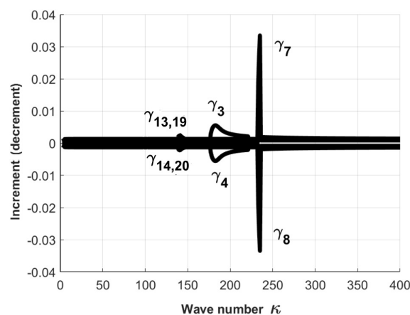
Fig. 15. The same as in Fig. 11, but at \theta = 90^\circ
