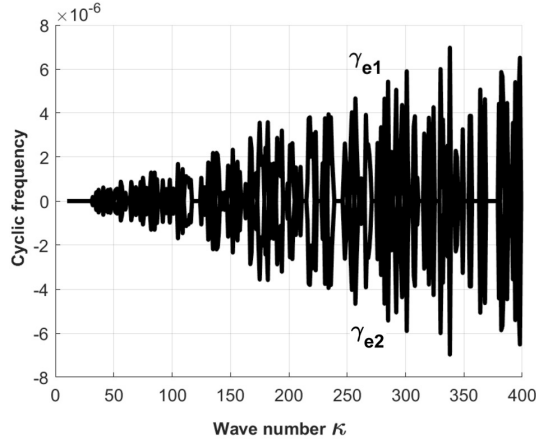
Fig. 7. The parameter \gamma_{e1} is the increment of growth, and \gamma_{e2} is the decrement of damping of the amplitude of ordinary electron plasmon-polaritons due to their pseudo-chaotic instability at \theta = 0^\circ
