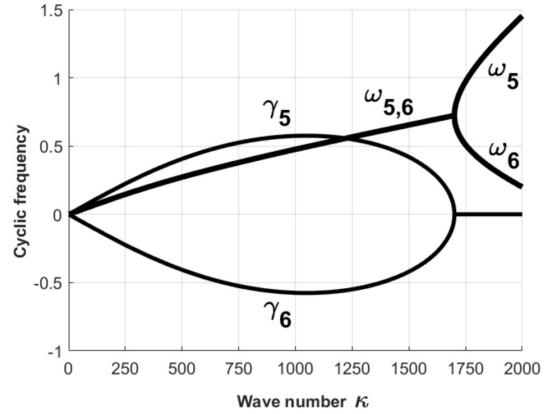
Fig. 2. Dispersion branches of hybrid plasmons at \theta = 0^\circ
