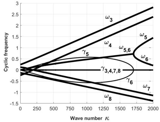
Fig. 3. The same as in Fig. 2, but at \theta = 30^\circ
