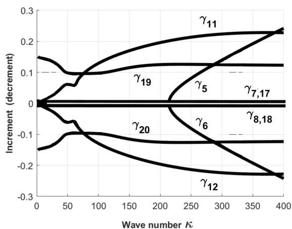
Fig. 11. The instability parameters of hybrid plasmon-polaritons at \theta = 30^\circ enlarged view
