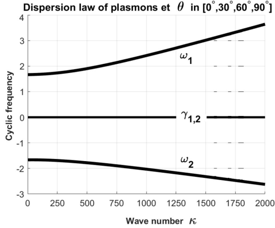
Fig. 1. Dispersion branches of ordinary plasmons in Ge
