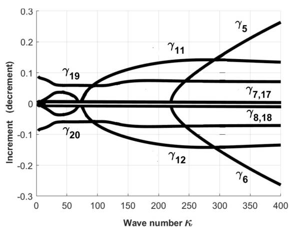
Fig. 13. The same as in Fig. 11, but at \theta = 60^\circ
