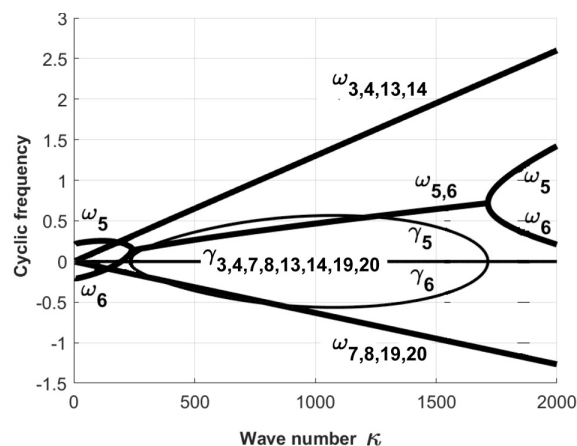
Fig. 14. The same as in Fig. 9, but at \theta = 90^\circ
