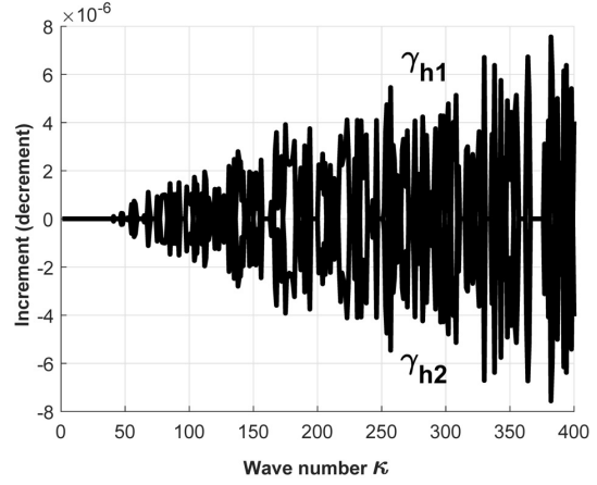
Fig. 8. The parameter \gamma_{h1} is the increment of growth, and \gamma_{h2} is the decrement of damping of the amplitude of ordinary hole plasmon-polaritons due to their pseudo-chaotic instability at \theta = 0^\circ
