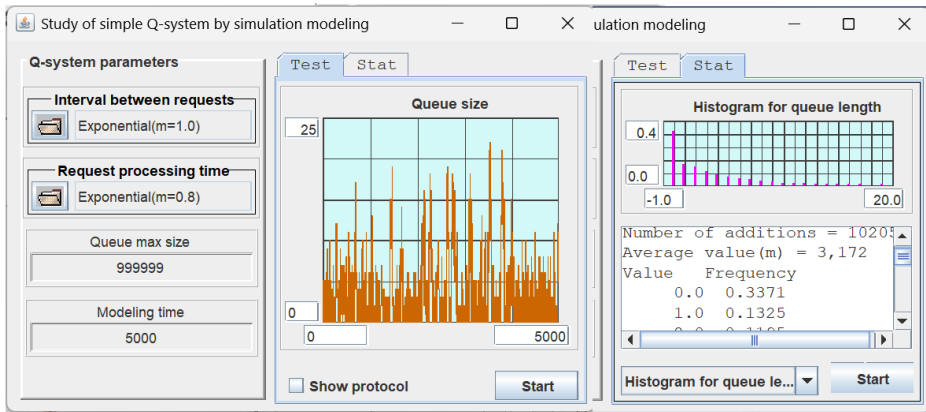
Fig. 3. Application for studying a simple Markov queueing system
